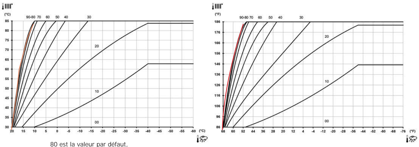
FIGURE 8-6 – Courbes de climat Kt
