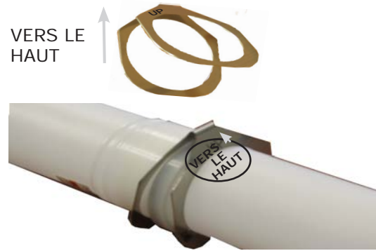
Figure 5-11 – Bride Natalini
