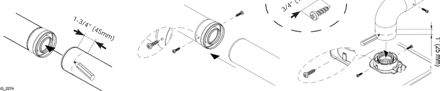
Figure 5-2 - Placement de Vis Coaxial
