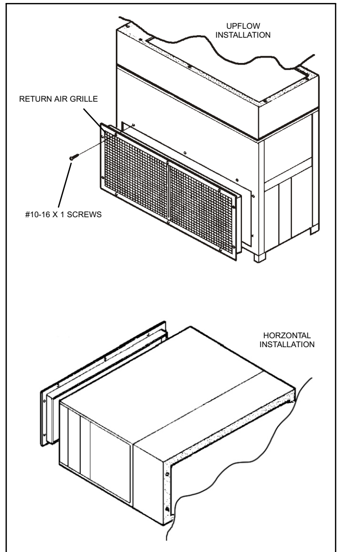
Figure 1. Typical Return Air Grille Installation
