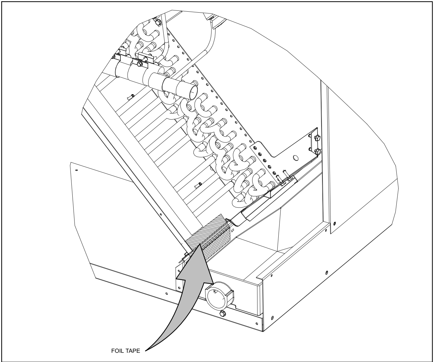
Figure 8. Applying Foil Tape to Coil Support
