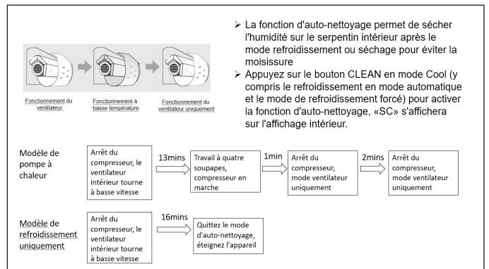
Figure 40. Auto nettoyant
