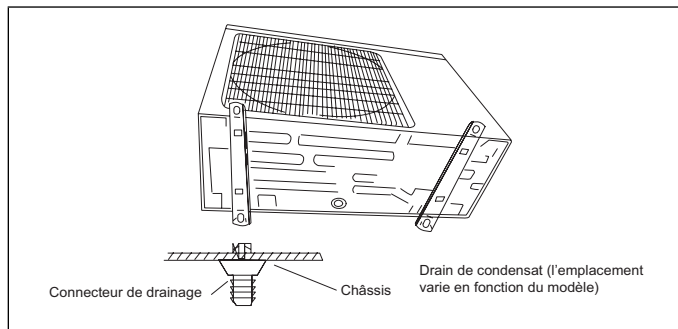
Figure 22. Drain de condensat
