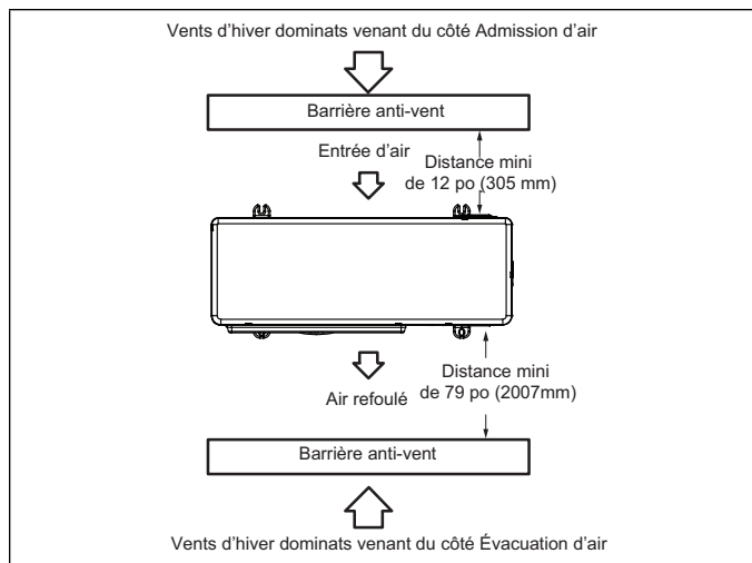
Figure 19. Barrière anti-vent
