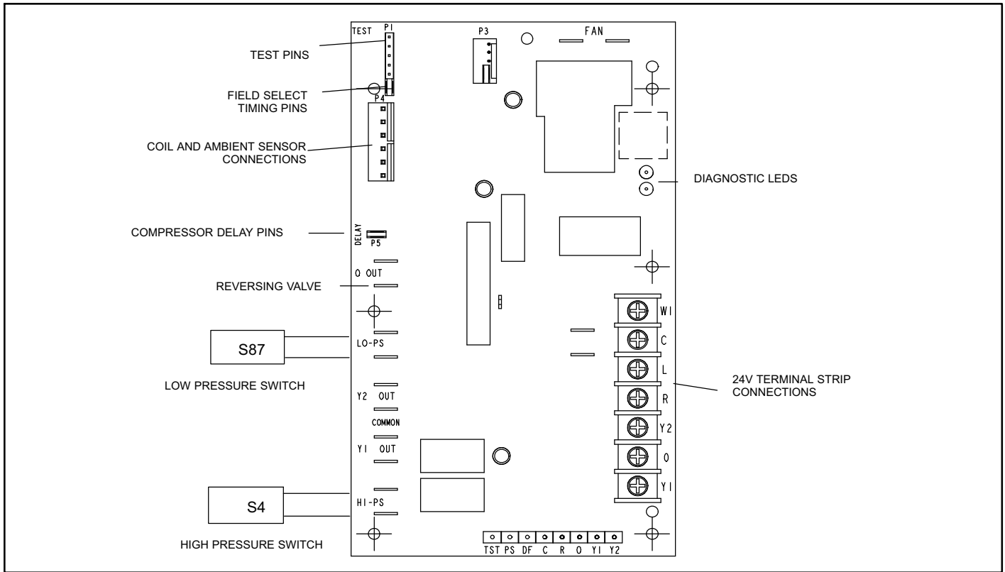
Figure 2. Defrost Control (100135-07)
