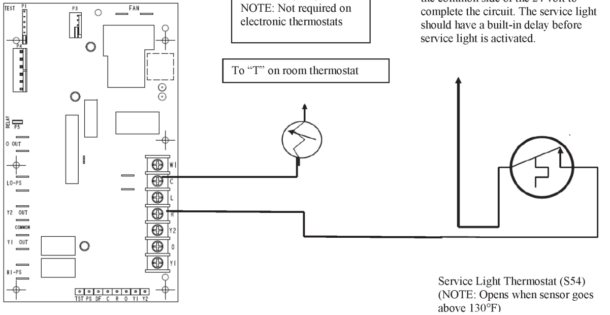
Figure 12. RT3 Sensor and Service Light Wiring
