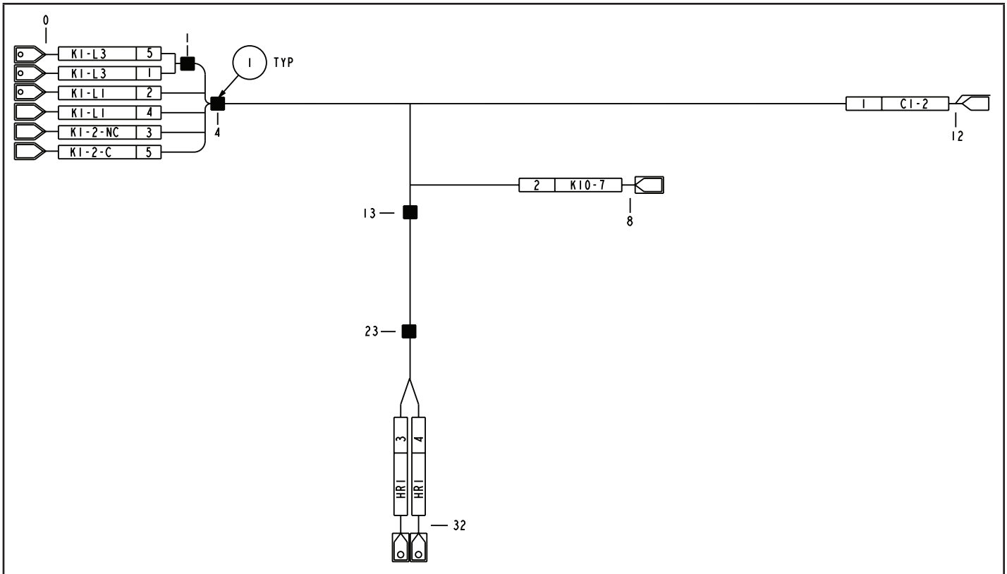
FIGURE 4. Factory-Installed Fan Power Harness (Must be Removed)
