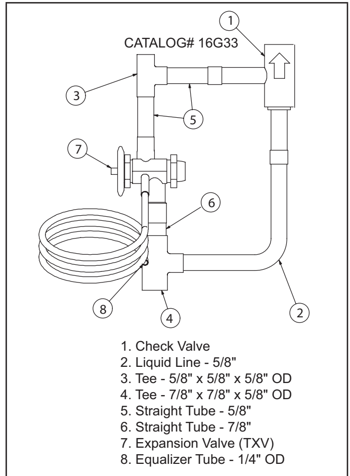
FIGURE 1. Component Layout
