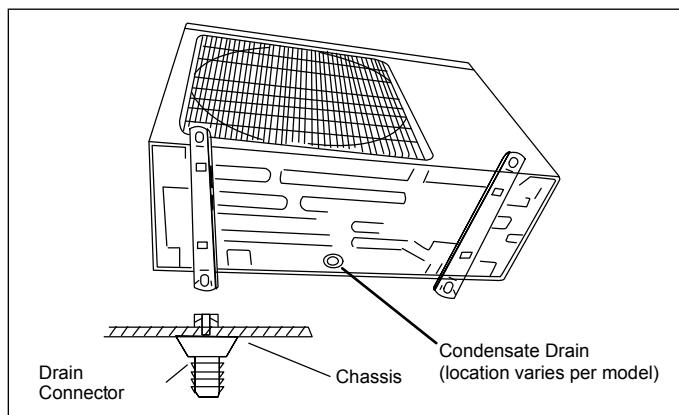
Figure 23. Condensate Drain
