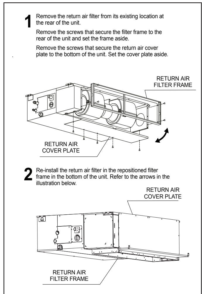
Figure 10. Field-Relocation of Return Air Filter (Typical) - Bottom Return Air
