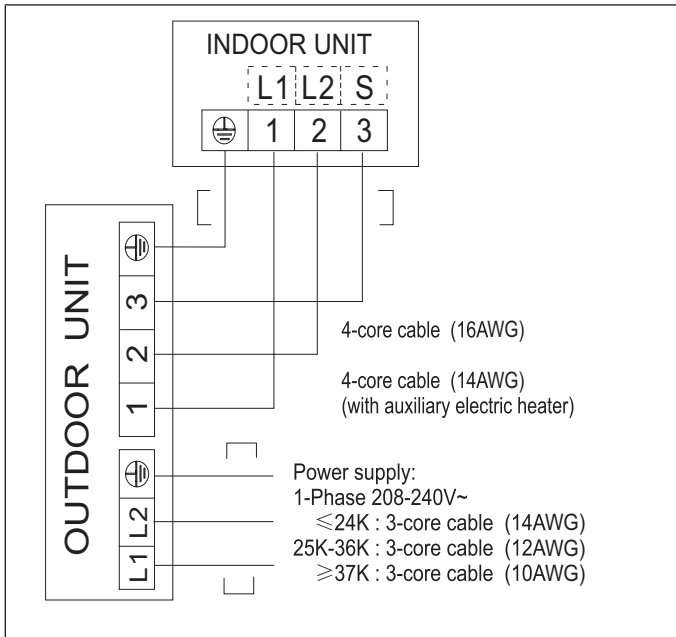
Figure 30. Single-Zone Wiring 9K, 12K, 18K and 24K
