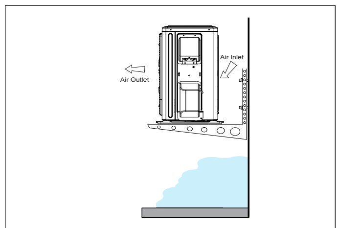
Figure 17. Outdoor Unit on Brackets above Snow Line
