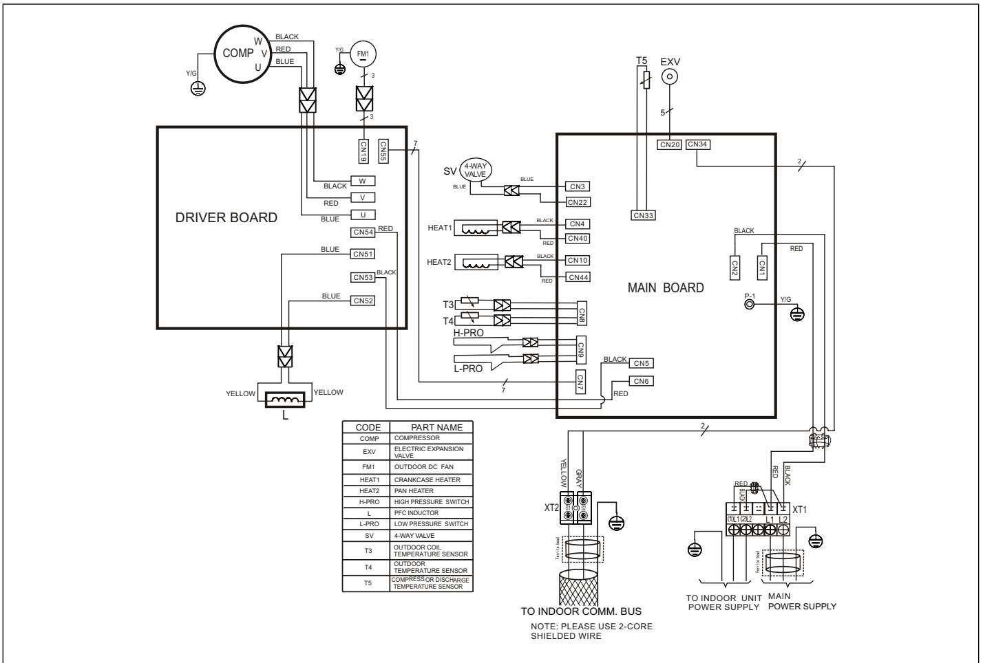
Figure 36. 208/230V MPB036S4S-*P Outdoor Unit Wiring Diagram
