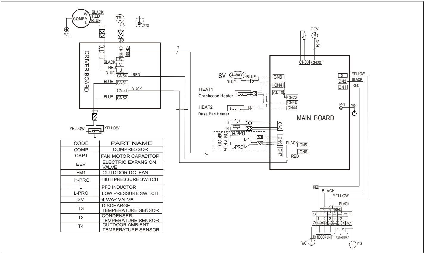
Figure 39. 208/230V MLA024S4S-*P Outdoor Unit Wiring Diagram
