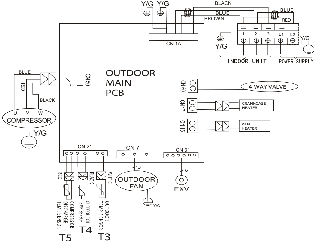
Figure 34. 208/230V MPB009S4S-*P and MPB012S4S-*P Outdoor Unit Wiring Diagram
