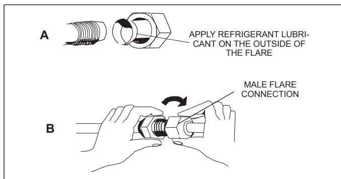
Figure 28. Making Connections (Male to Female Connection)
