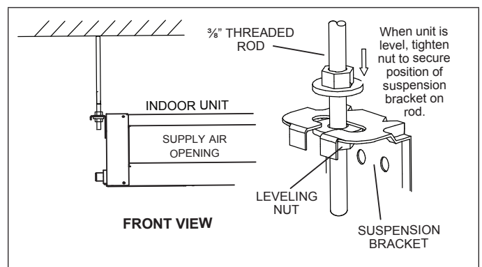
Figure 8. Suspending Hardware
