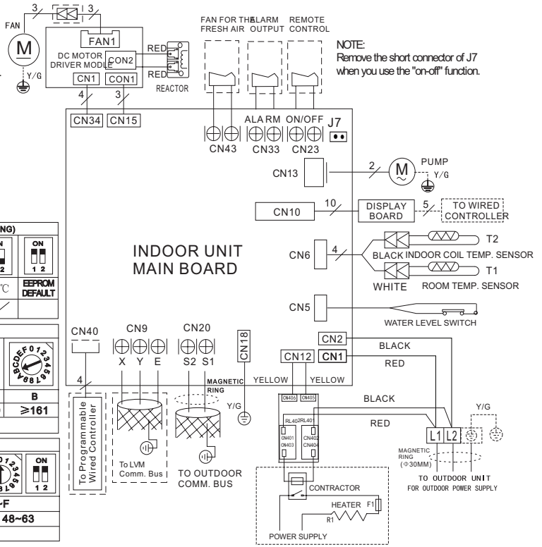
Figure 33. MMDB036S4-*P and MMDB048S4-*P Ducted Units Wiring Diagram
