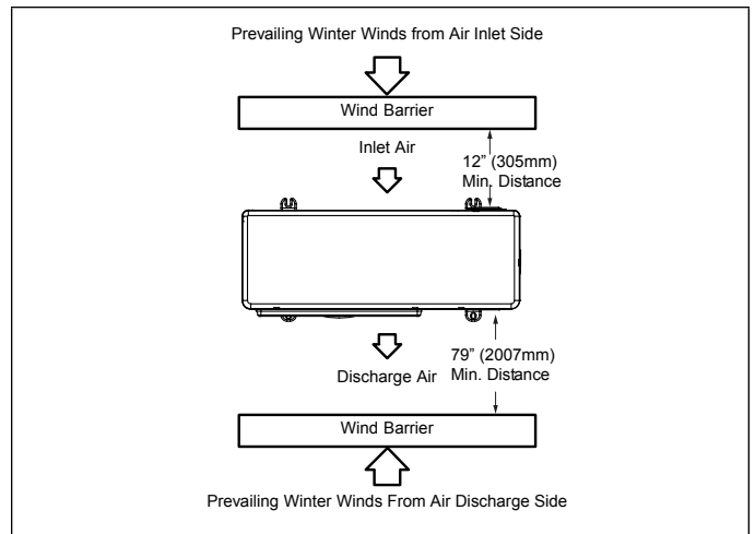
Figure 20. Wind Barrier
