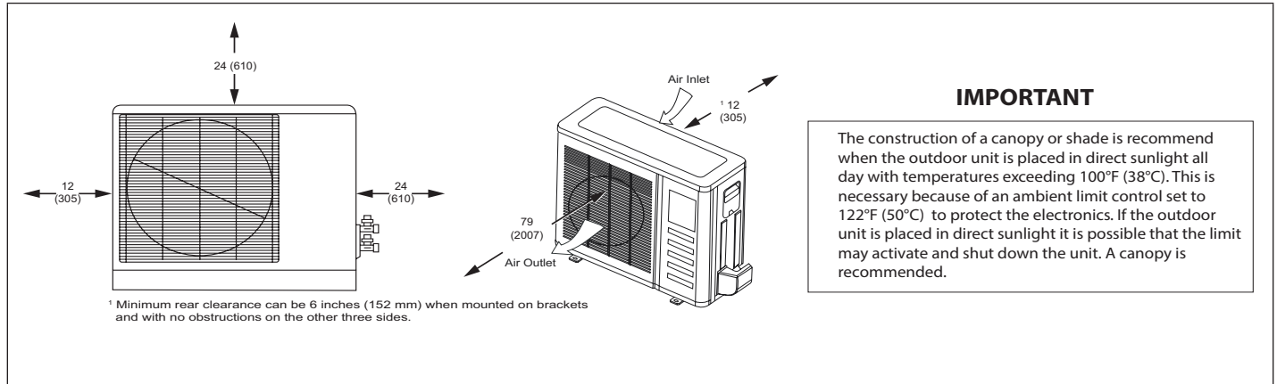
Figure 5. Outdoor Unit Clearances - Inches (mm)
