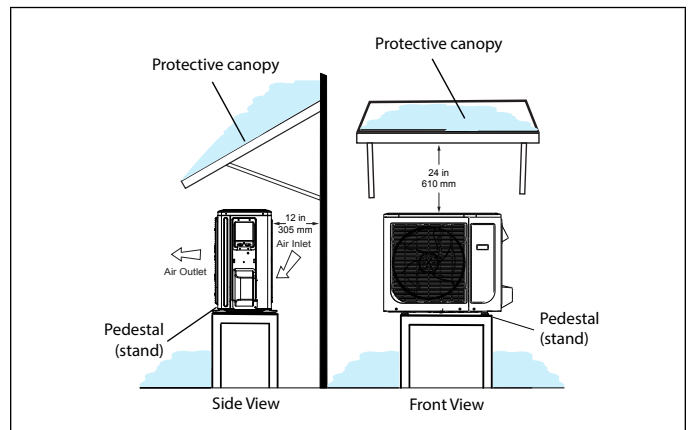
Figure 16. Outdoor Unit on Pedestal (Stand) and Protective Canopy
