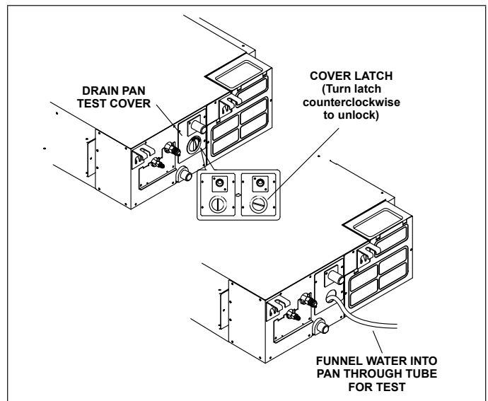
Figure 14. Condensate Drain Test
