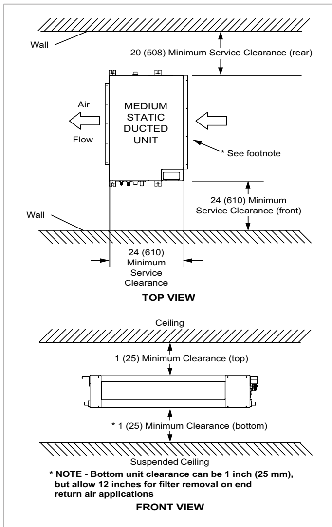
Figure 6. Indoor Unit Clearances - Inches (mm)
