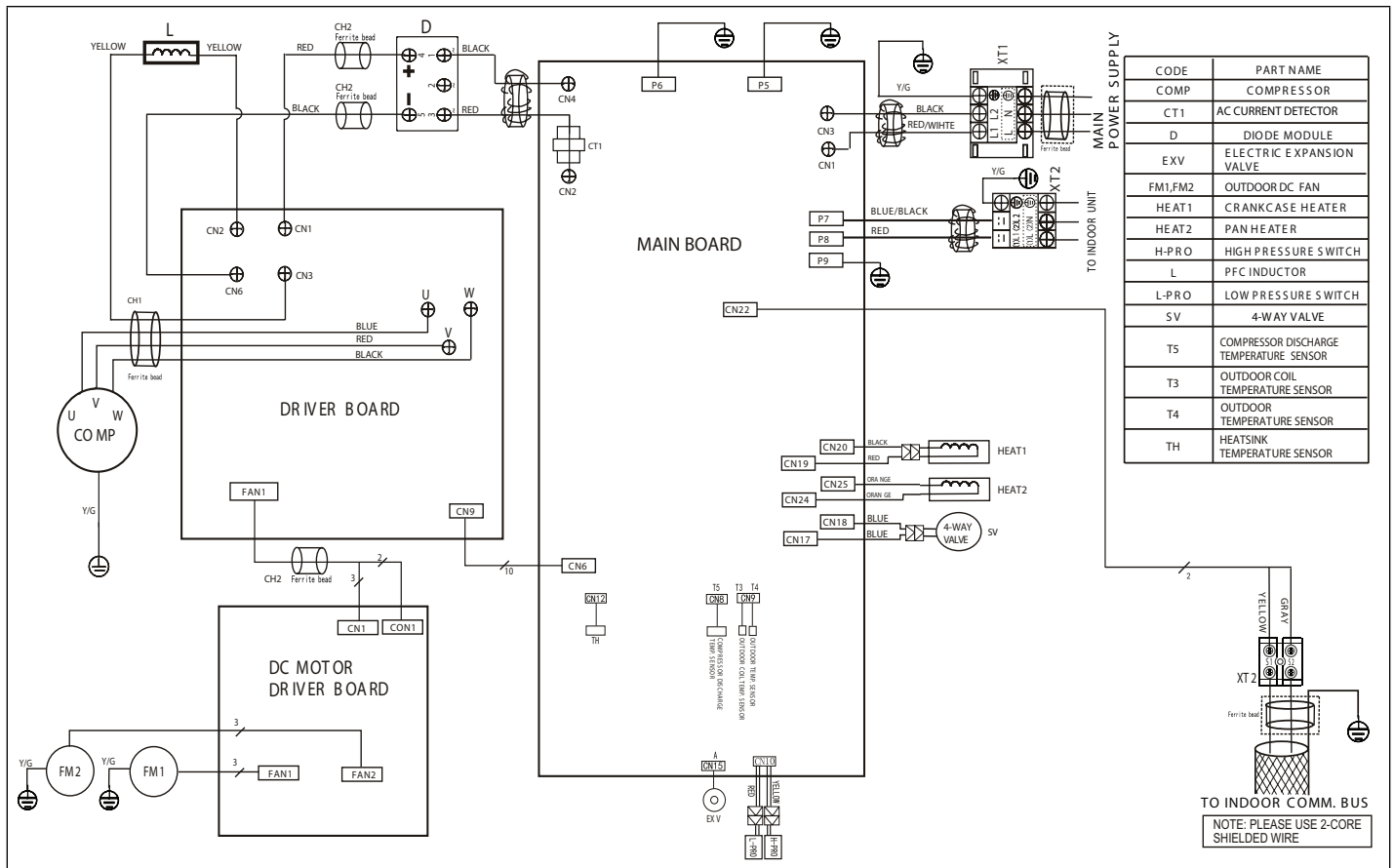
Figure 37. 208/230V MPB048S4S-*P Outdoor Unit Wiring Diagram
