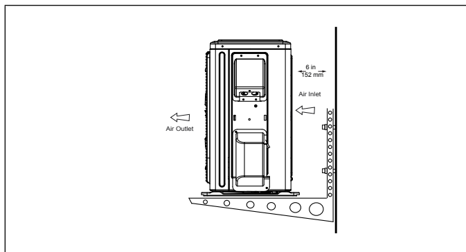
Figure 26. Securing Outdoor Unit to Brackets
