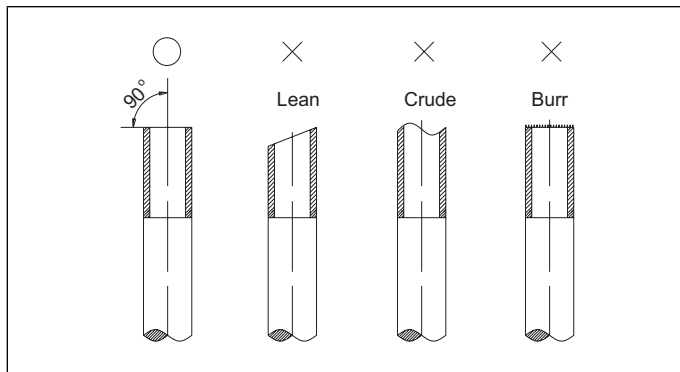
Figure 27. Cutting Pipe
