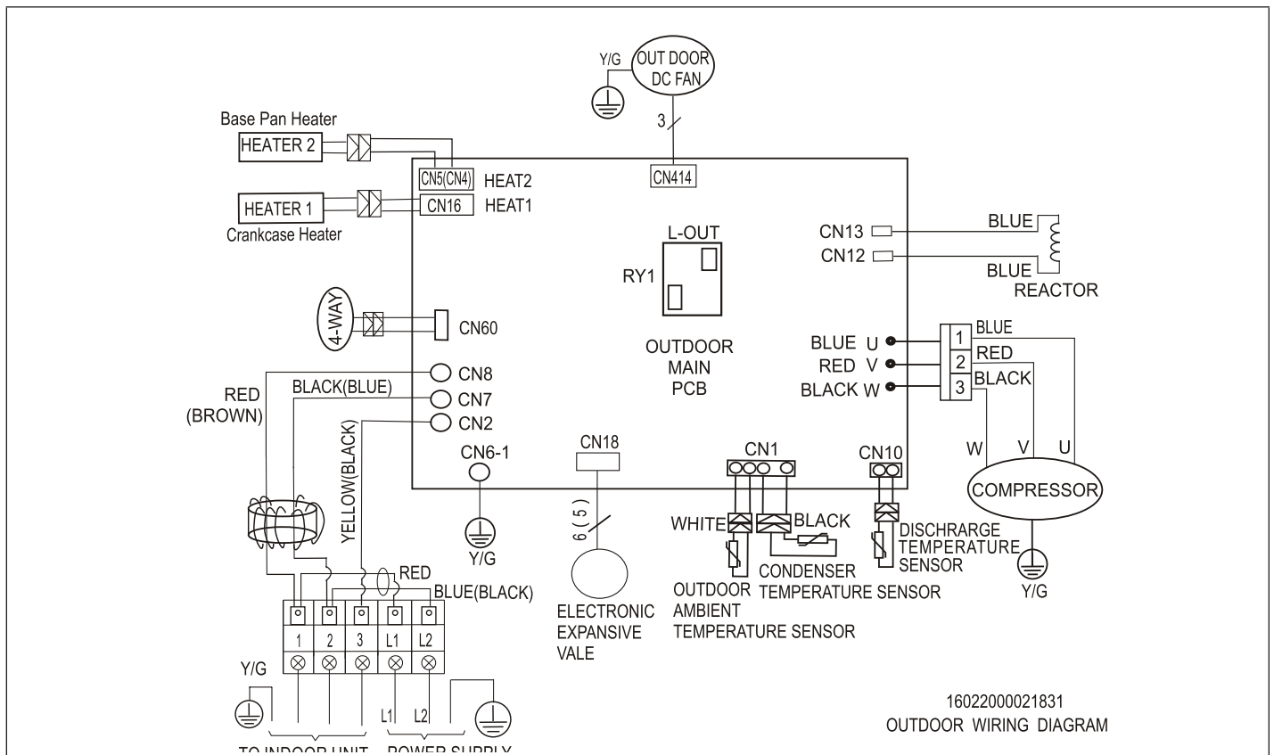
Figure 38. 208/230V MLA009, 012 and 018S4S-*P Outdoor Unit Wiring Diagram
