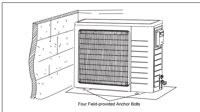
Figure 24. Securing Outdoor Unit to Slab
