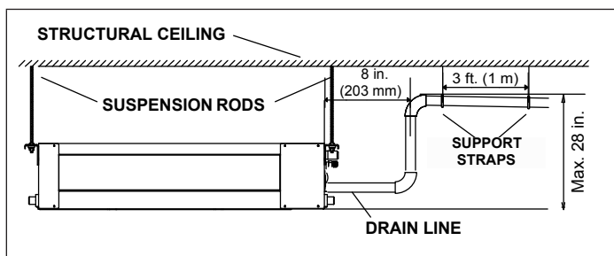
Figure 13. Condensate Drain with Factory Condensate Pump
