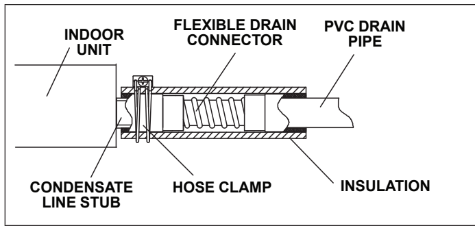
Figure 11. Condensate Gravity Drain Option
