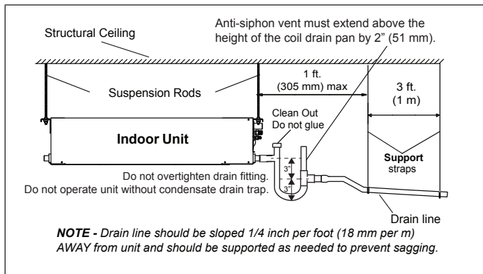
Figure 12. Slope Condensate Drain
