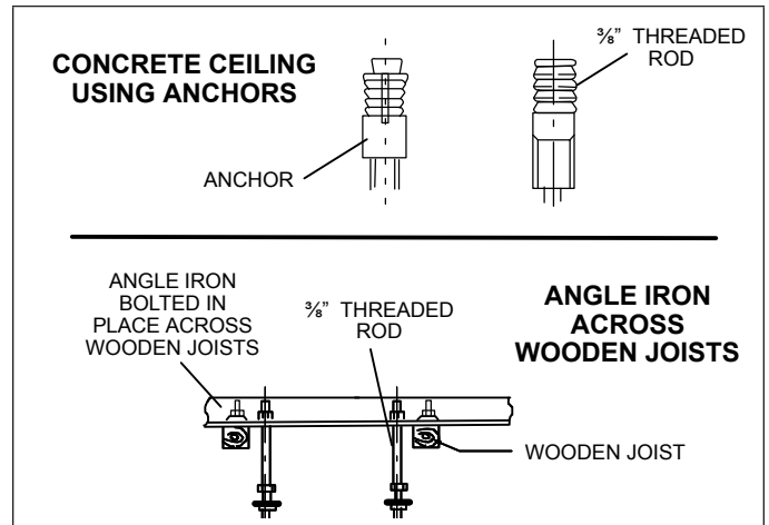
Figure 7. Suspending Methods
