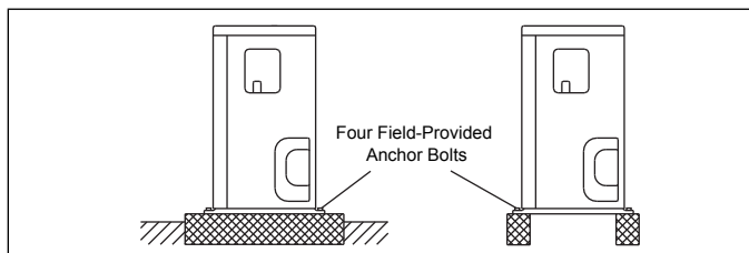
Figure 25. Securing Outdoor Unit to Rails
