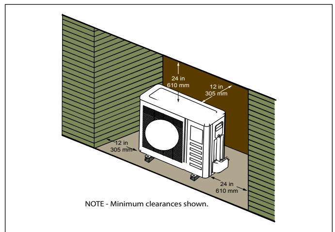
Figure 22. Unit installed in Alcove
