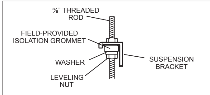
Figure 9. Isolation Grommet
