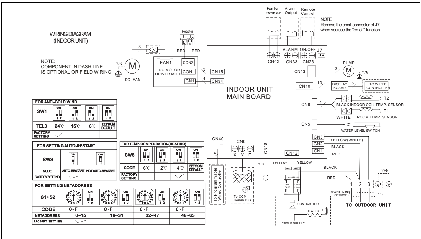
Figure 32. MMDB009S4-*P, MMDB012S4-*P, MMDB018S4-*P and MMDB024S4-*P Ducted Units Wiring Diagram
