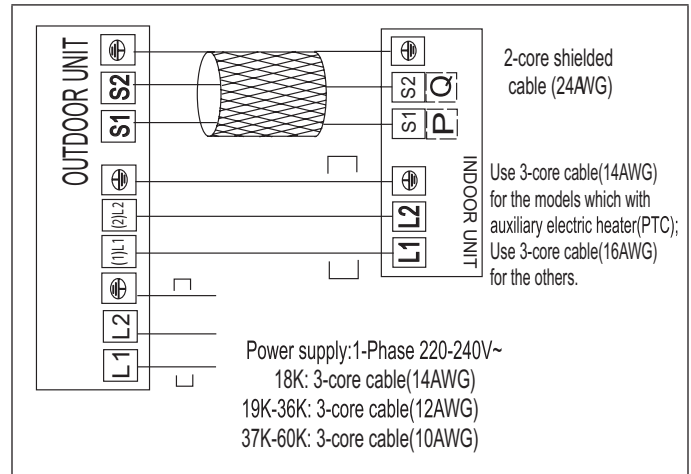
Figure 31. Single-Zone Wiring 36K and 48K
