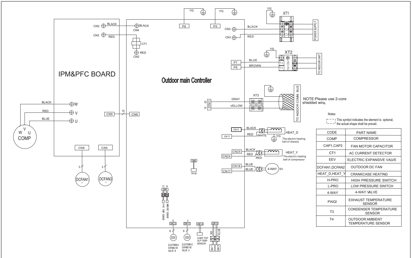
Figure 40. 208/230V MLB036S4S-*P and MLB048S4S-*P Outdoor Unit Wiring Diagram
