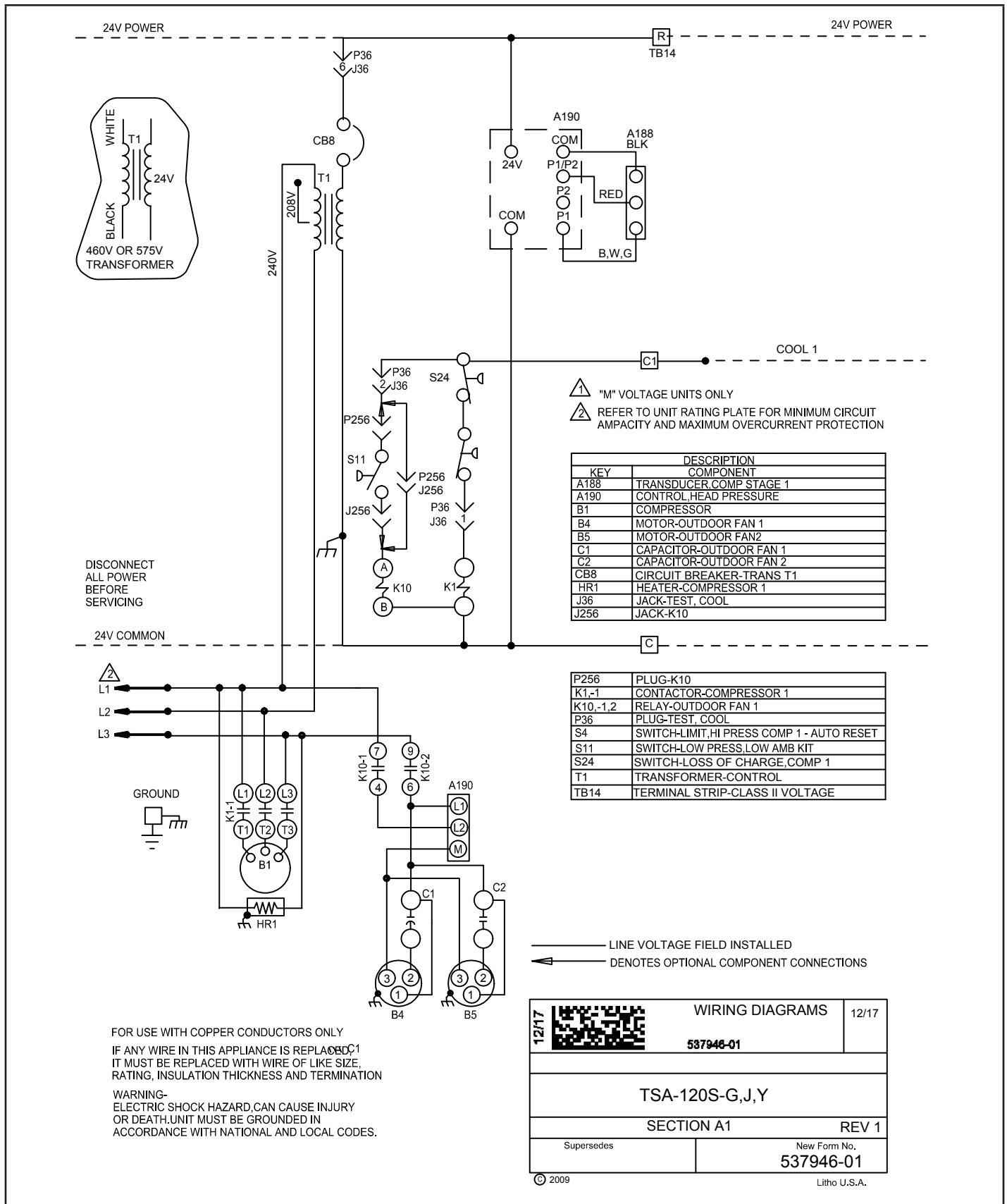
FIGURE 3. Wiring Diagram – TSA 120S
