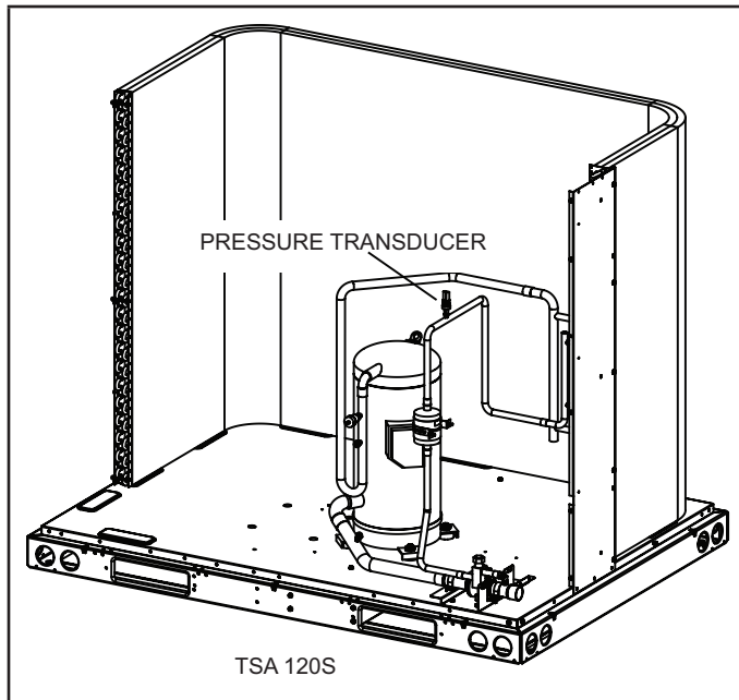
FIGURE 2. Pressure Transducer Location
