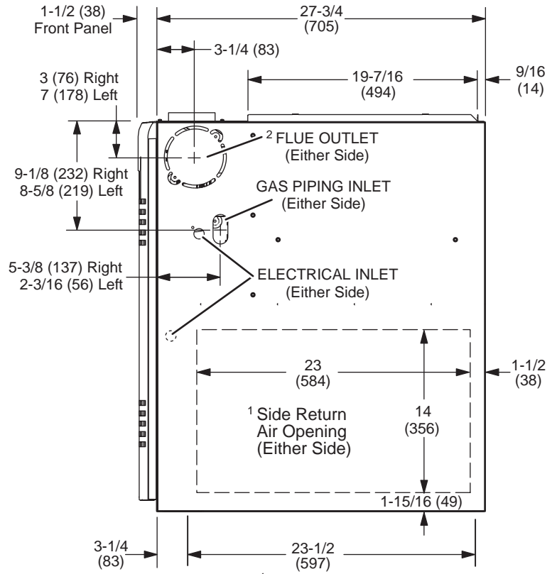
1 Bottom Return Air Opening SIDE VIEW
