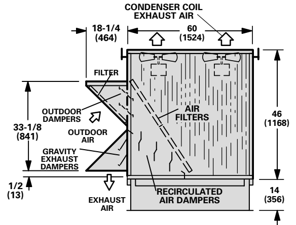
CONDENSER SECTION END VIEW
