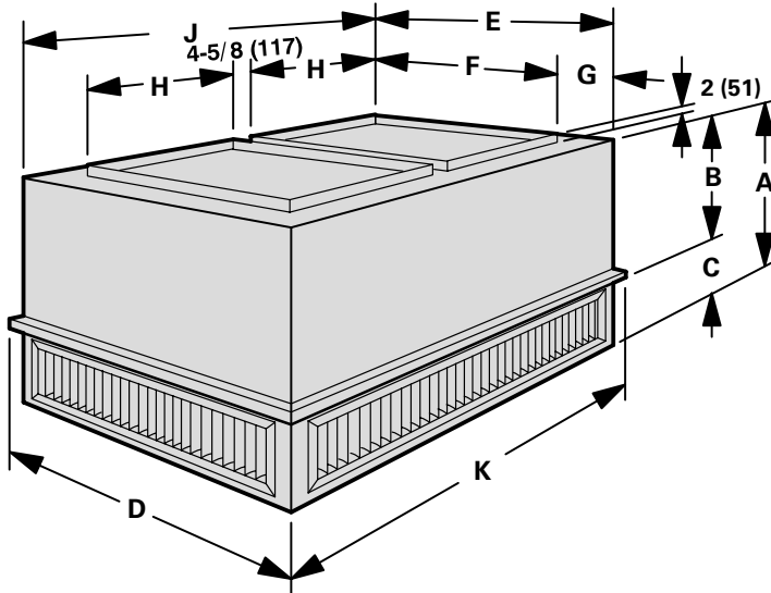
RTD11-135, RTD11-185 & RTD11-275 STEP-DOWN CEILING DIFFUSERS
