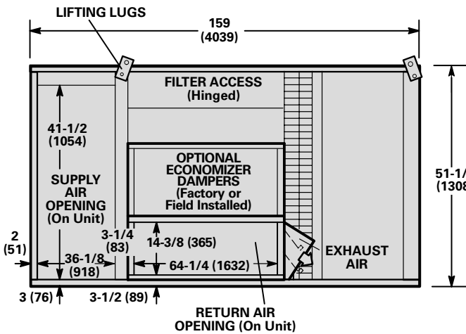
BACK VIEW
