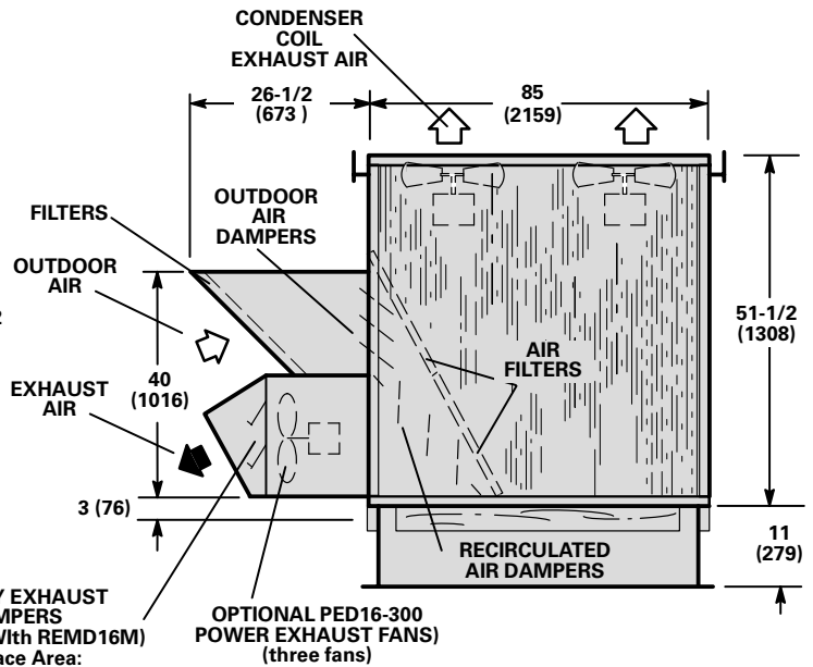
CONDENSER SECTION END VIEW
