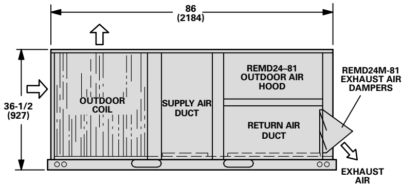
BACK VIEW With Horizontal Supply & Return Air Openings
