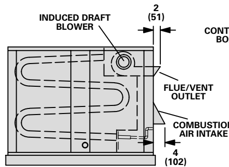
LEFT END VIEW HEAT SECTION
