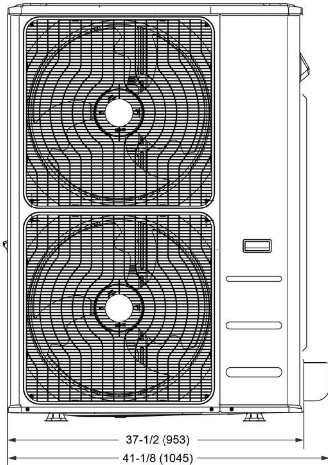
FRONT VIEW
