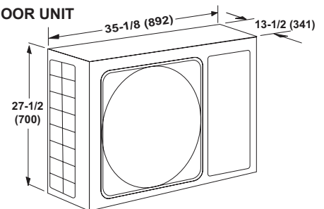
OUTDOOR UNIT
