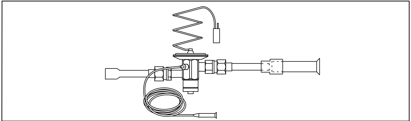
FIGURE 2. Chatleff-Style CTXV Assembly – Assembled
