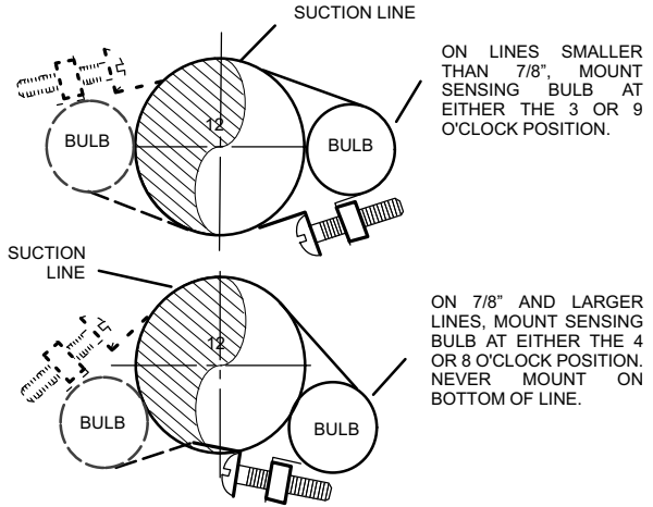
FIGURE 4. Check / Expansion Valve Replacement Procedure – Continued
