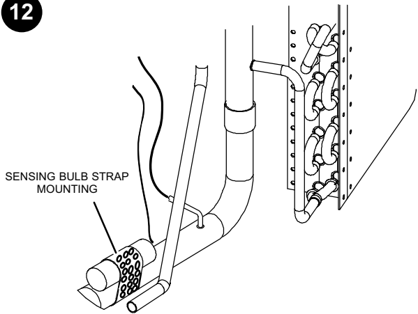
FIGURE 4. Check / Expansion Valve Replacement Procedure – Continued
