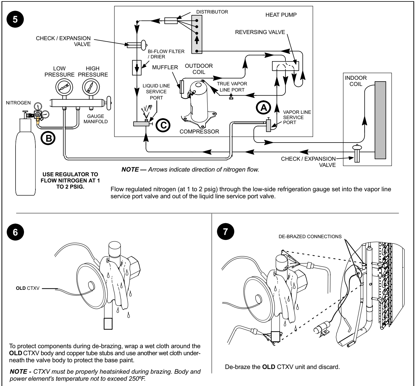
FIGURE 4. Check / Expansion Valve Replacement Procedure – Continued
