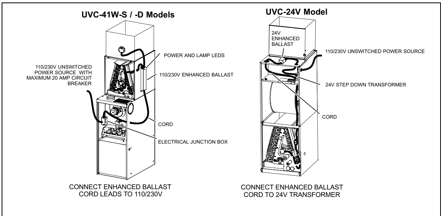
Figure 13. Preferred Power Connections
