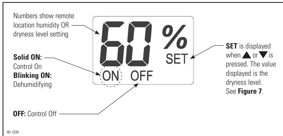
Figure 3. Remote Control LCD Display
