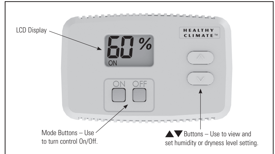
Figure 1. Control Display and User Buttons
