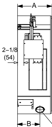
3 (76) FRESH AIR INTAKE OPENING
