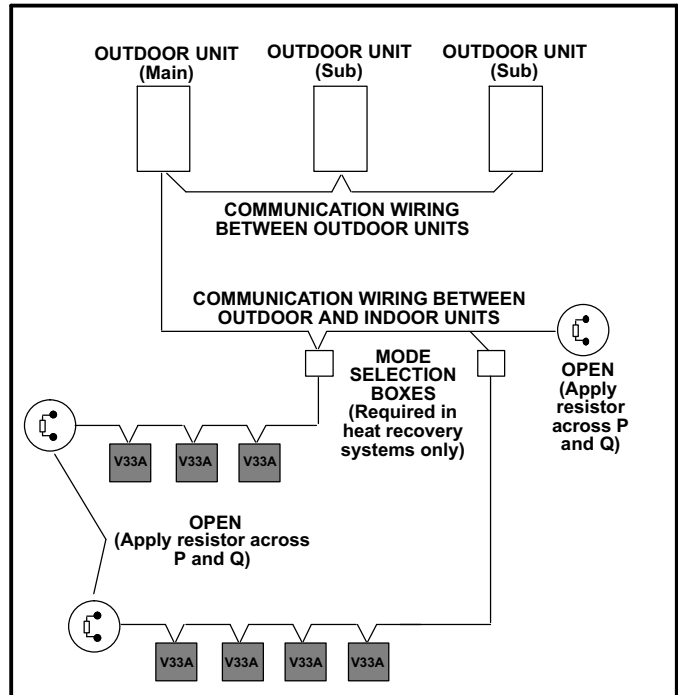
Figure 11. Typical Series Wiring of Indoor Units (with resistors)
