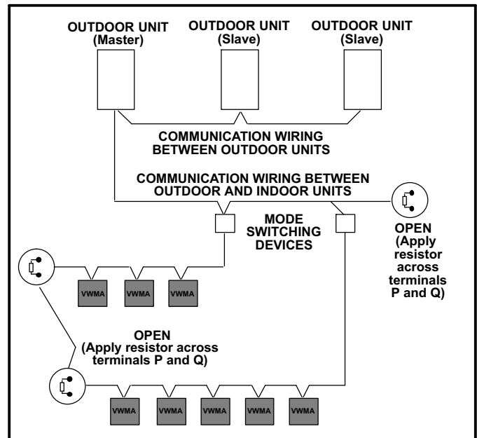
Figure 13. Typical Series Wiring of Indoor Units (with resistors)
