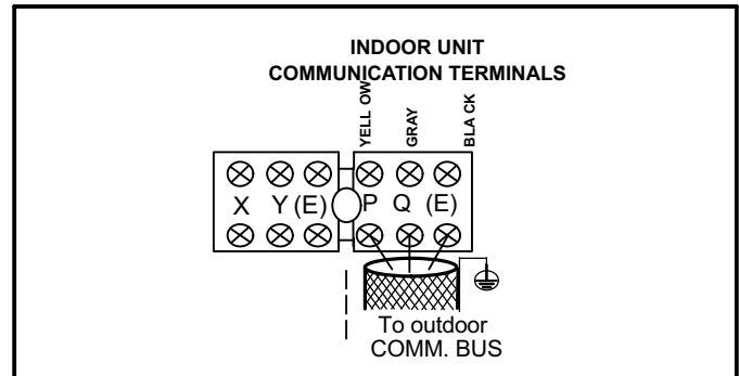
Figure 12. Typical Communications Wiring
