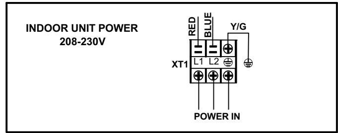
Figure 11. Typical Power Wiring
