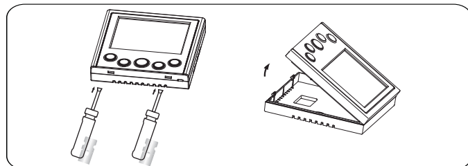
Figure 3. Remove cover from wallplate
