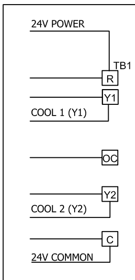
CONNECTION SCHEME FOR KCA, KGA AND KHA 092 THROUGH 150 UNITS WITHOUT ECONOMIZER ONLY
