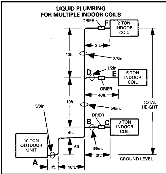
Figure 22. Liquid Plumbing
