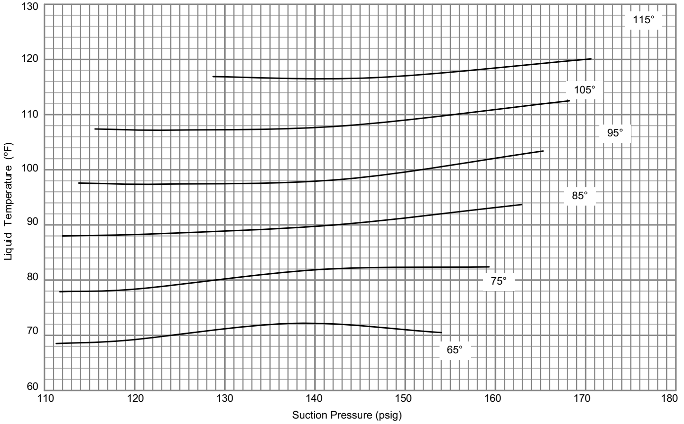
LGH/LCH180 VAV CHARGING CURVES CIRCUIT 1 Outdoor Temperature (°F)
