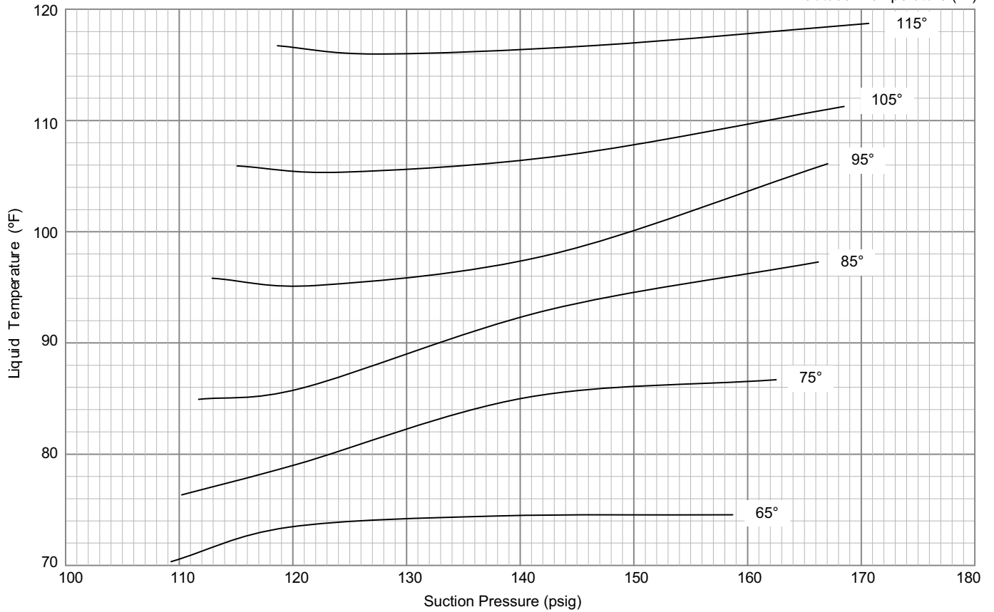
LGH/LCH156 CAV/STAGED REHEAT CHARGING CURVES CIRCUIT 1 - 580907-02 Outdoor Temperature (°F)
