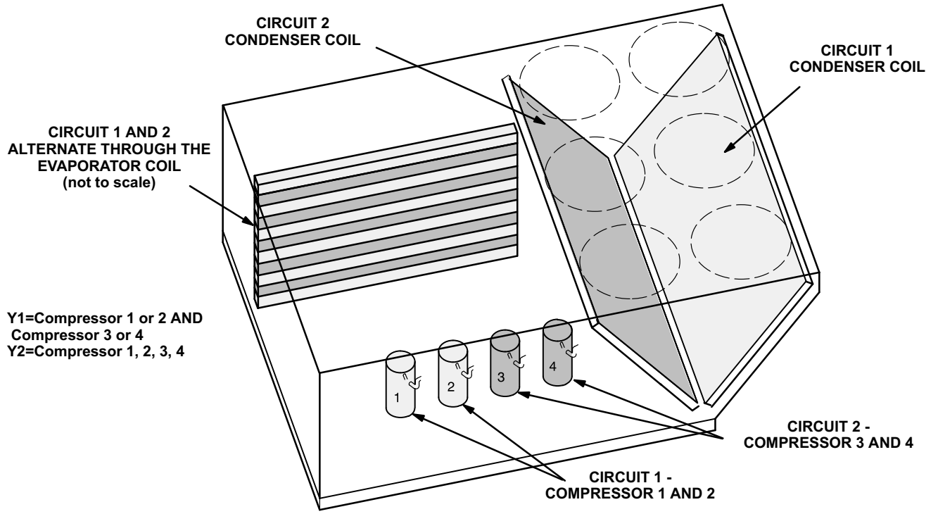
180U & 240U COMPRESSOR DETAIL
