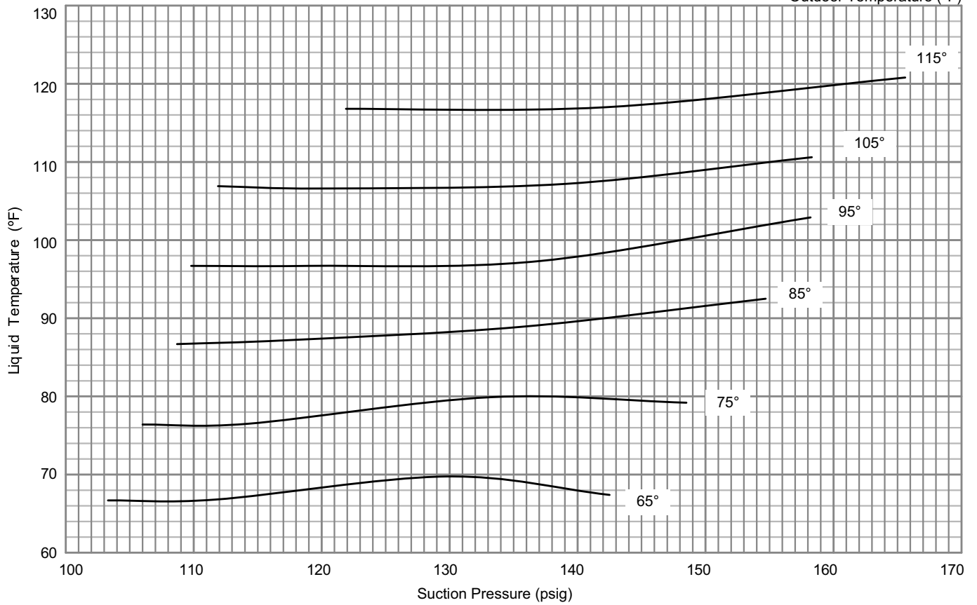
LGH/LCH180 CAV/STAGED REHEAT CHARGING CURVES CIRCUIT 2 Outdoor Temperature (°F)
