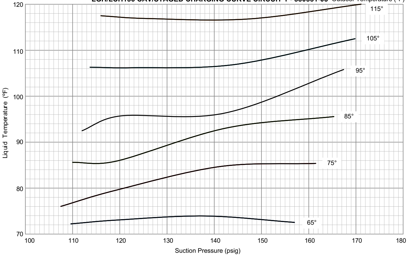
LGH/LCH156 CAV/STAGED CHARGING CURVE CIRCUIT 2 - 580551-03 Outdoor Temperature (°F)
