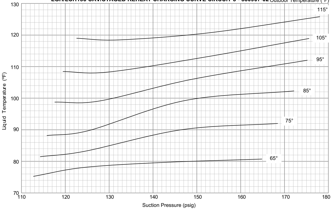
LGH/LCH156 CAV/STAGED REHEAT CHARGING CURVE CIRCUIT 3 - 580907-02 Outdoor Temperature (°F)
