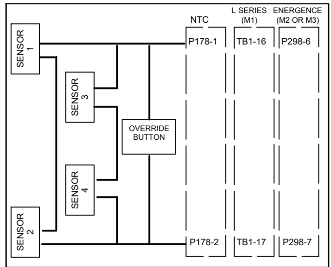
Figure 8. Wiring Standard Sensors for Averaging
