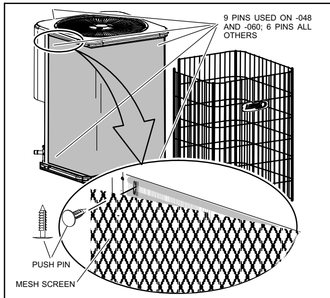
Figure 18. Cleaning Debris from Mesh
