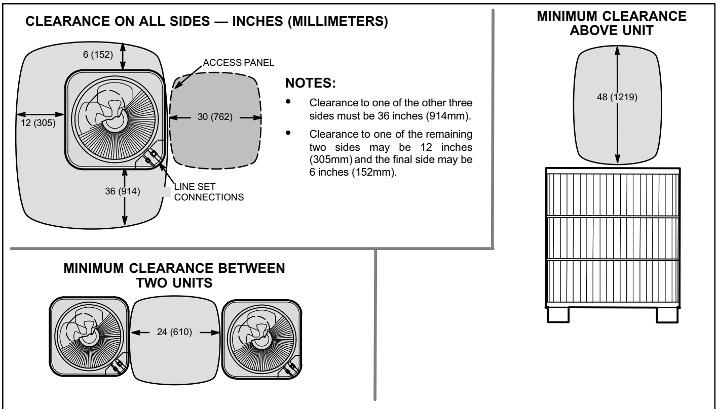
Figure 2. Installation Clearances
