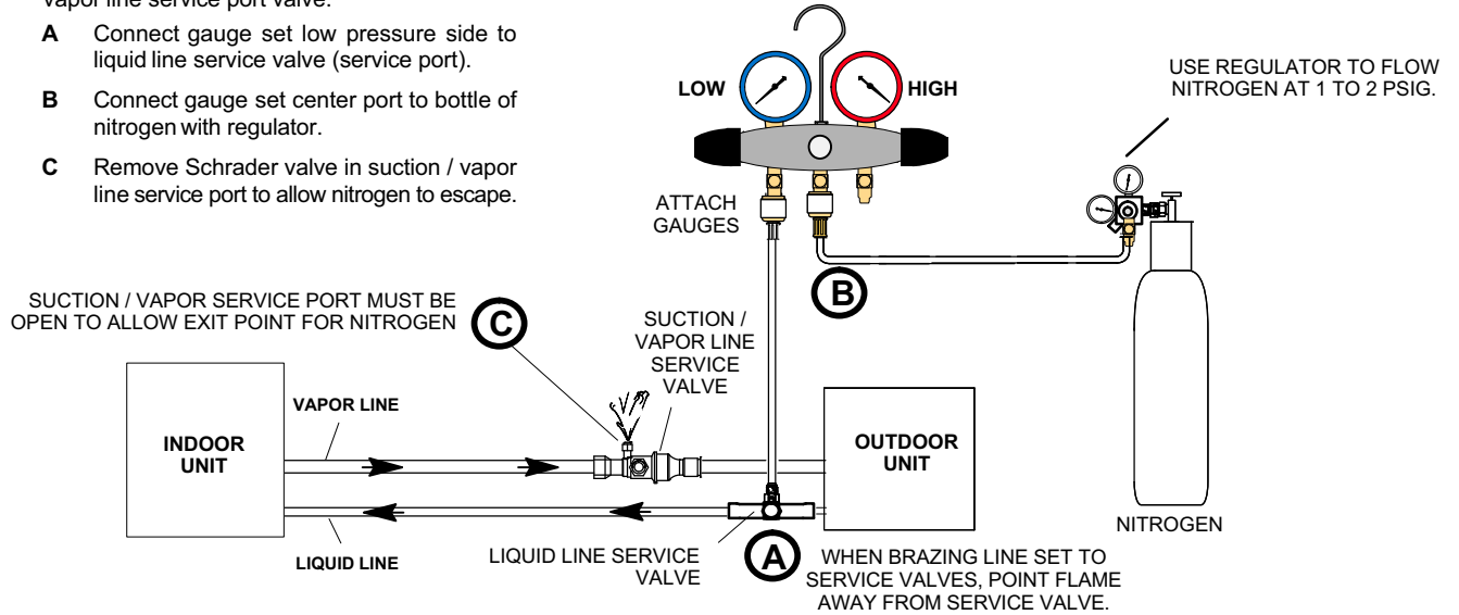
Figure 5. Brazing Procedures
