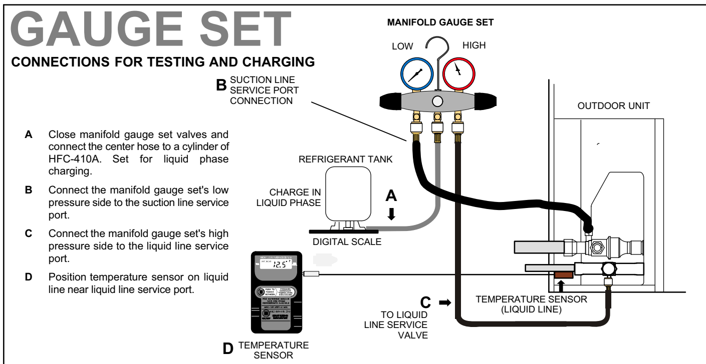
Figure 12. Manifold Gauge Set Setup and Connections
