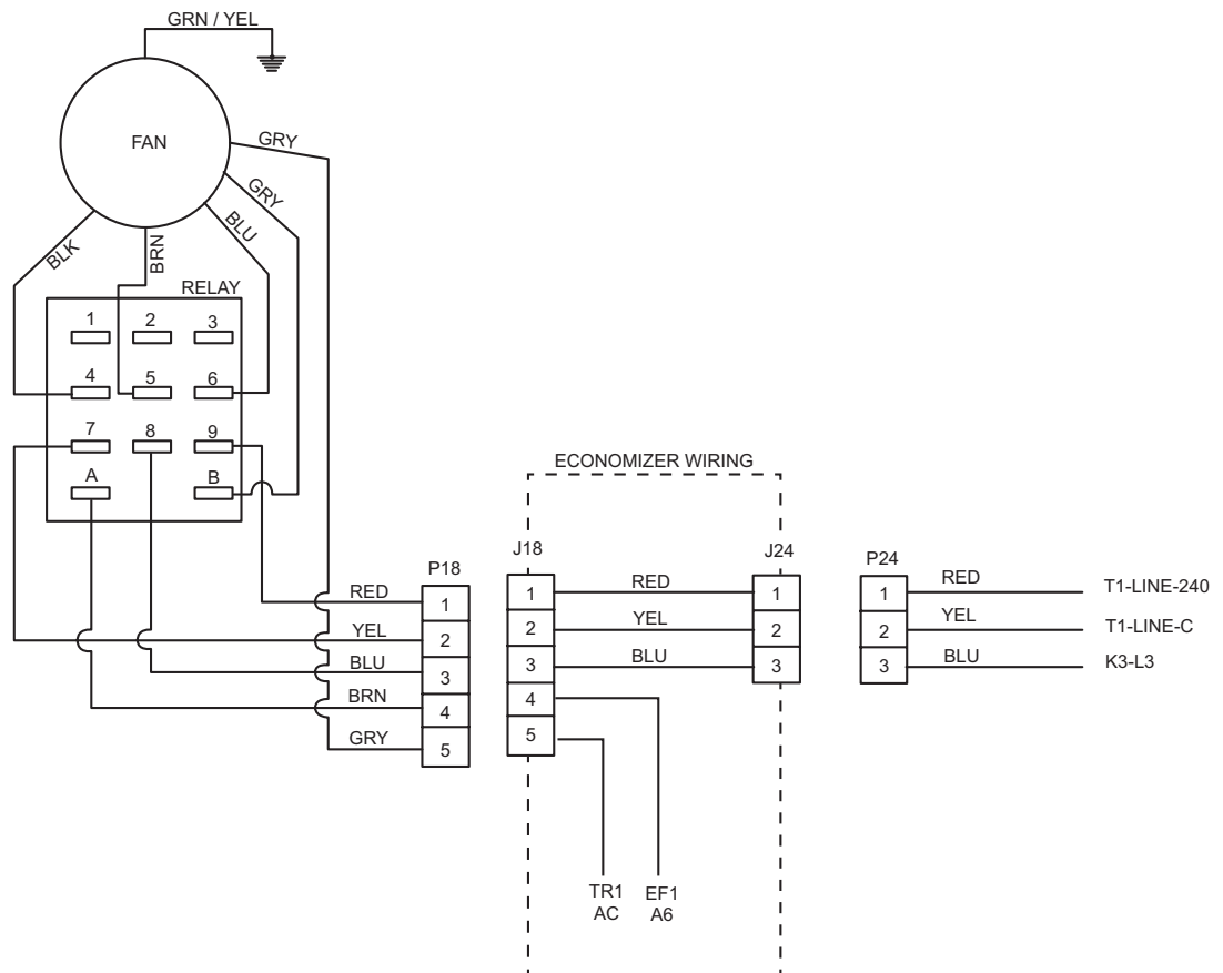
Figure 7 - Wiring Diagram for 460v 3PH
