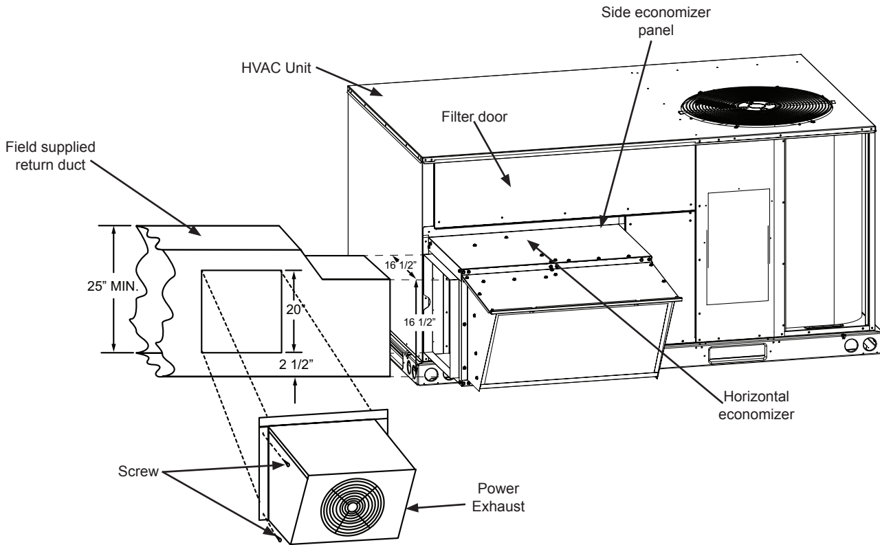
Figure 5 - 036-060 Unit Installation
