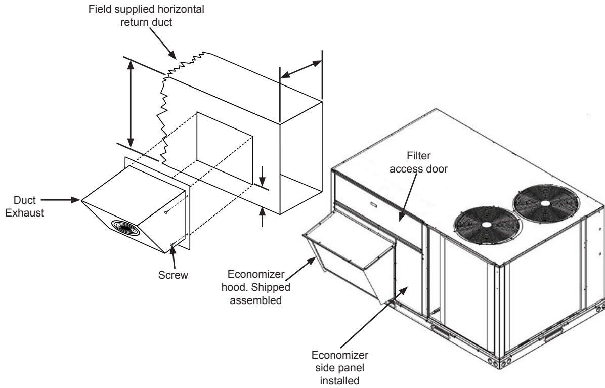
Figure 6 - 072-150 Unit Installation
