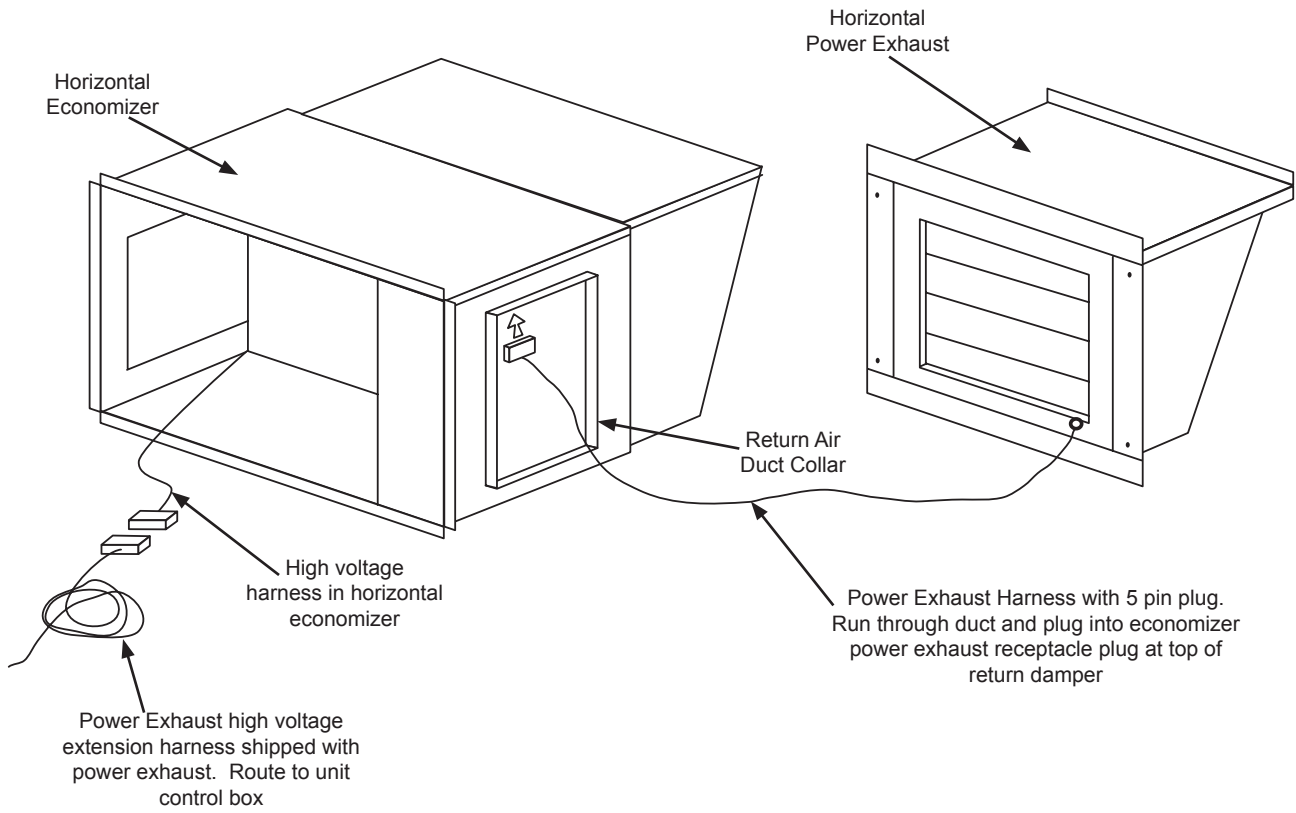
Figure 4 - (036-060 Size Shown)
