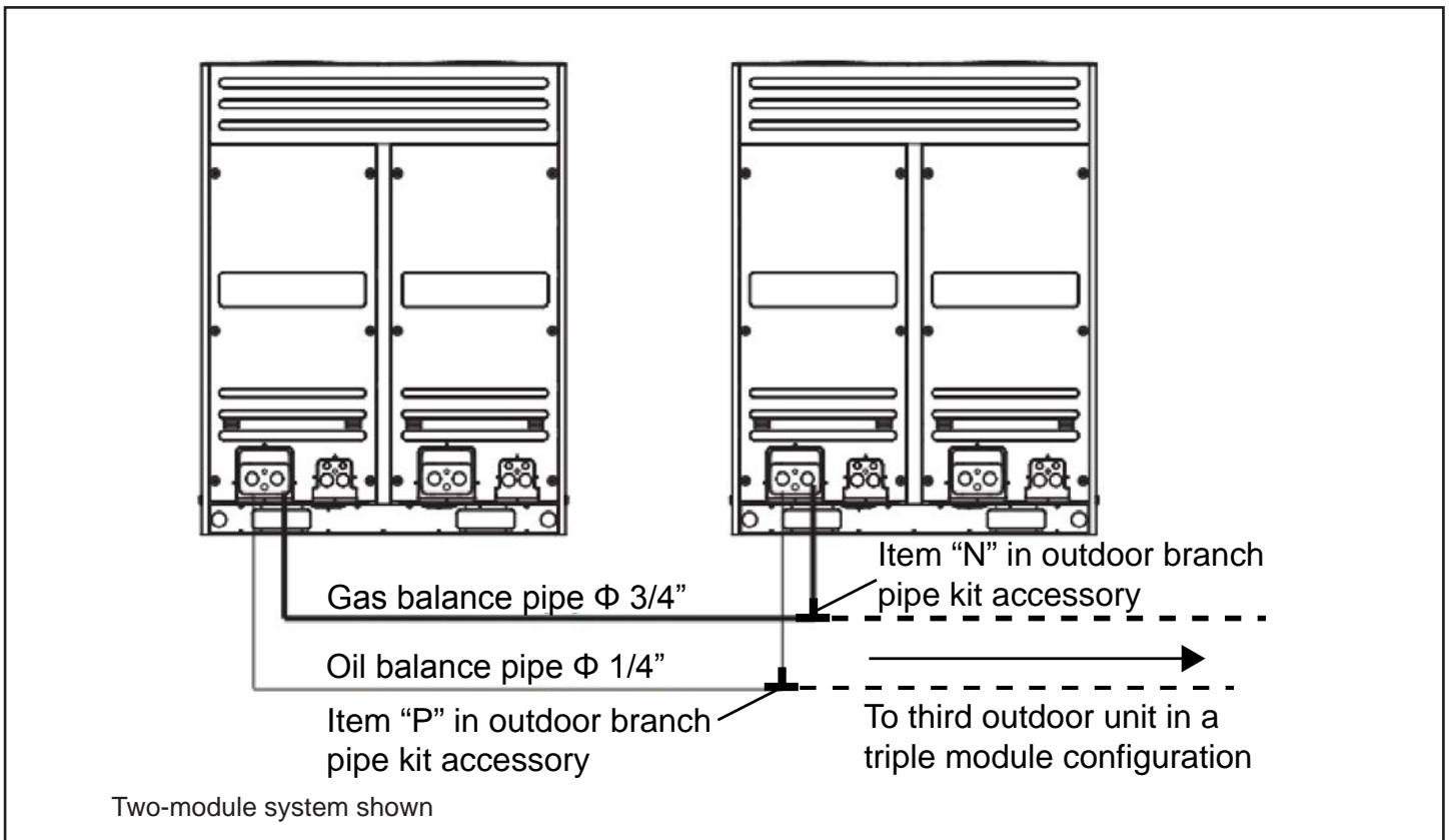
Figure 18. Connective Piping Sizes for Manifolder Outdoor Units
