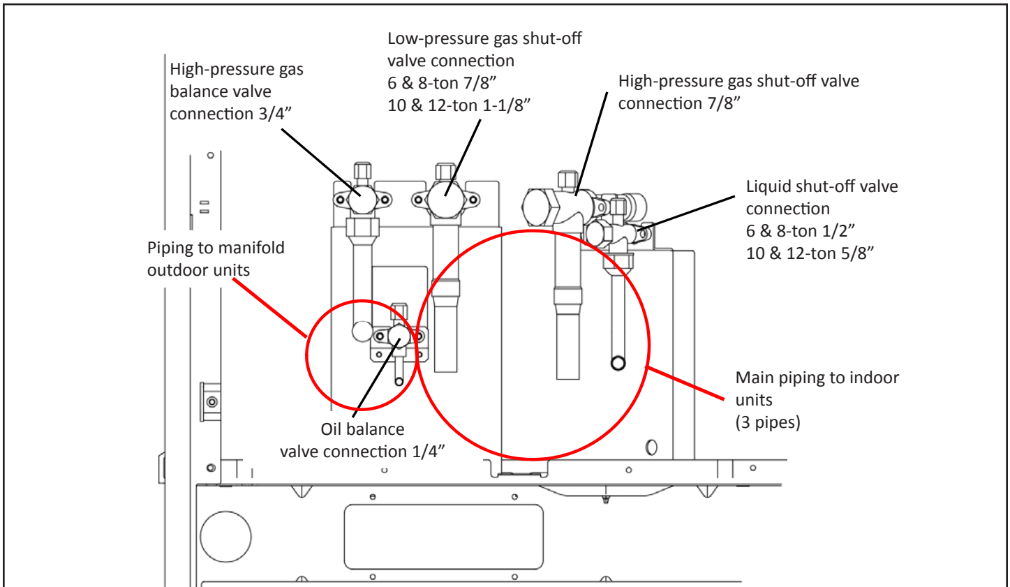
Figure 17. Heat Recovery Internal Valve Layout
