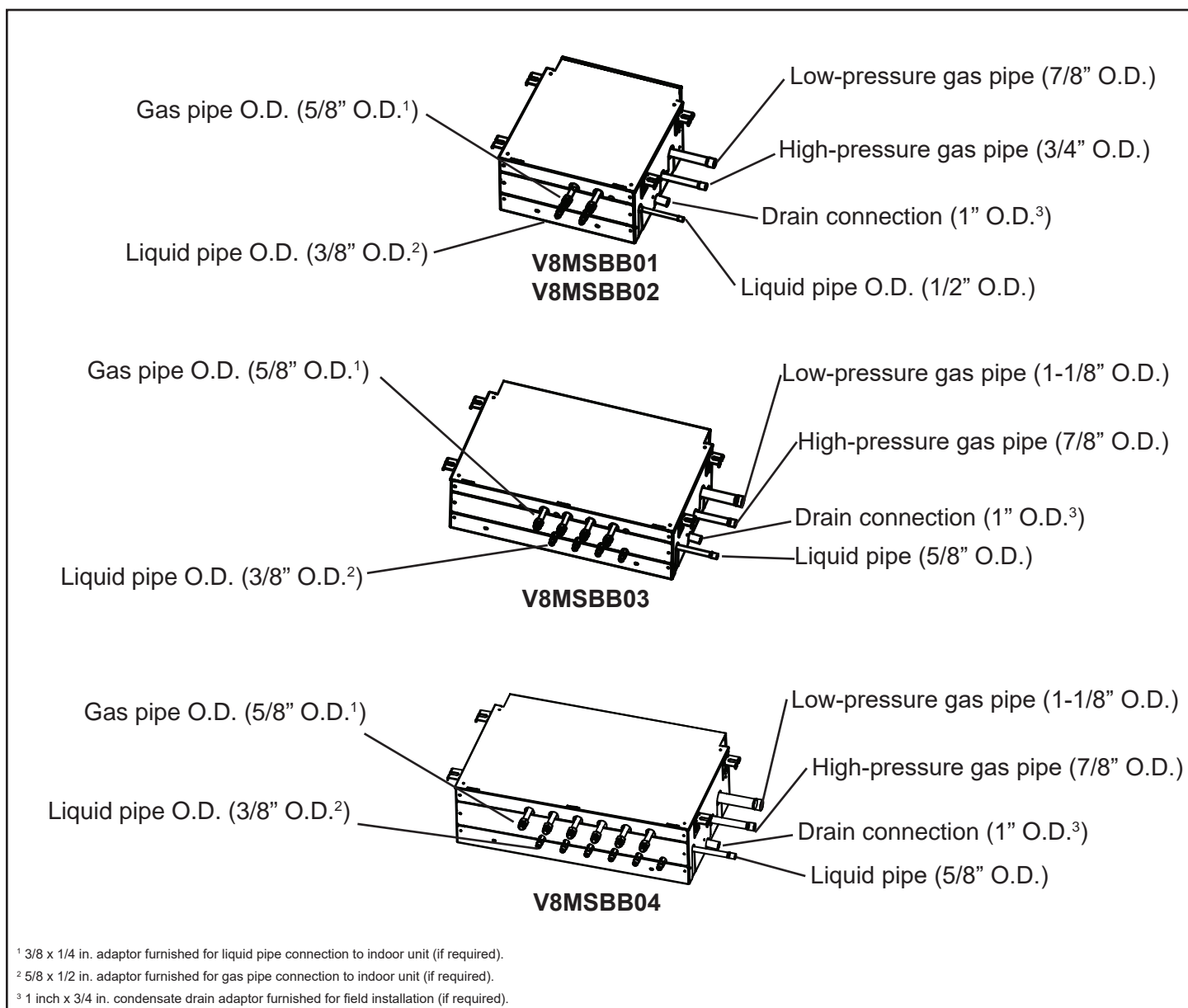
Figure 20. Mode Selection Box Piping Dimensions
