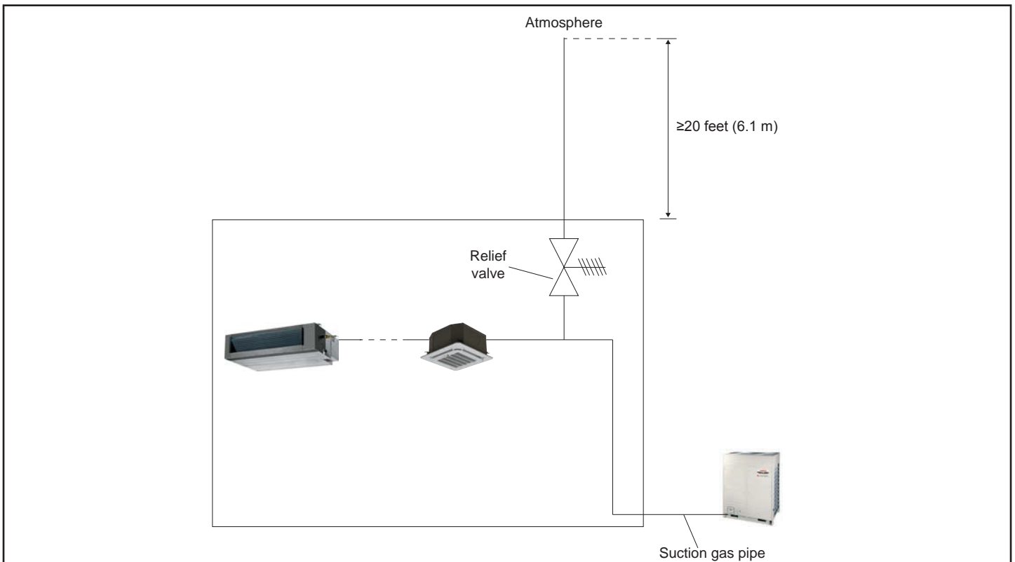
Figure 15. Refrigerant Discharge
