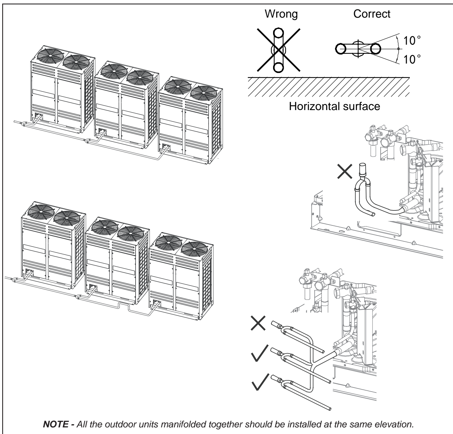
Figure 16. Connecting Manifolded Units
