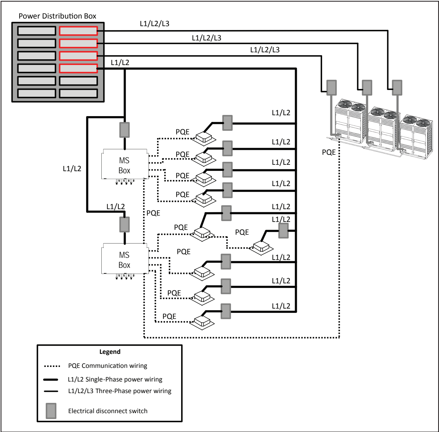
Figure 27. VRA Typical Power Wiring
