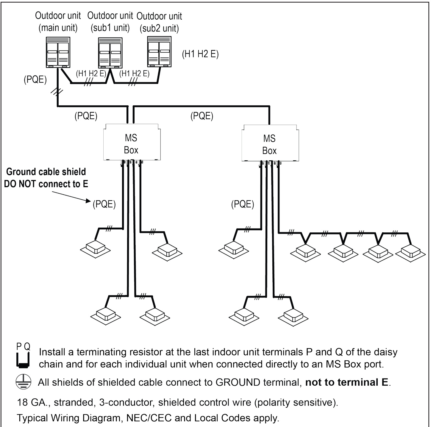
Figure 28. VRA Heat Recovery Typical Control Wiring
