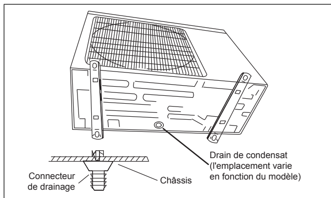
Figure 31. Drain de condensat
