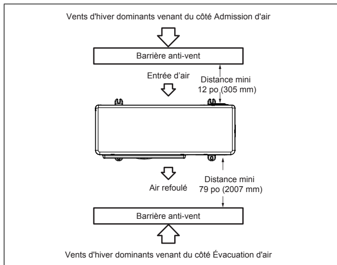
Figure 28. Barrière anti-vent
