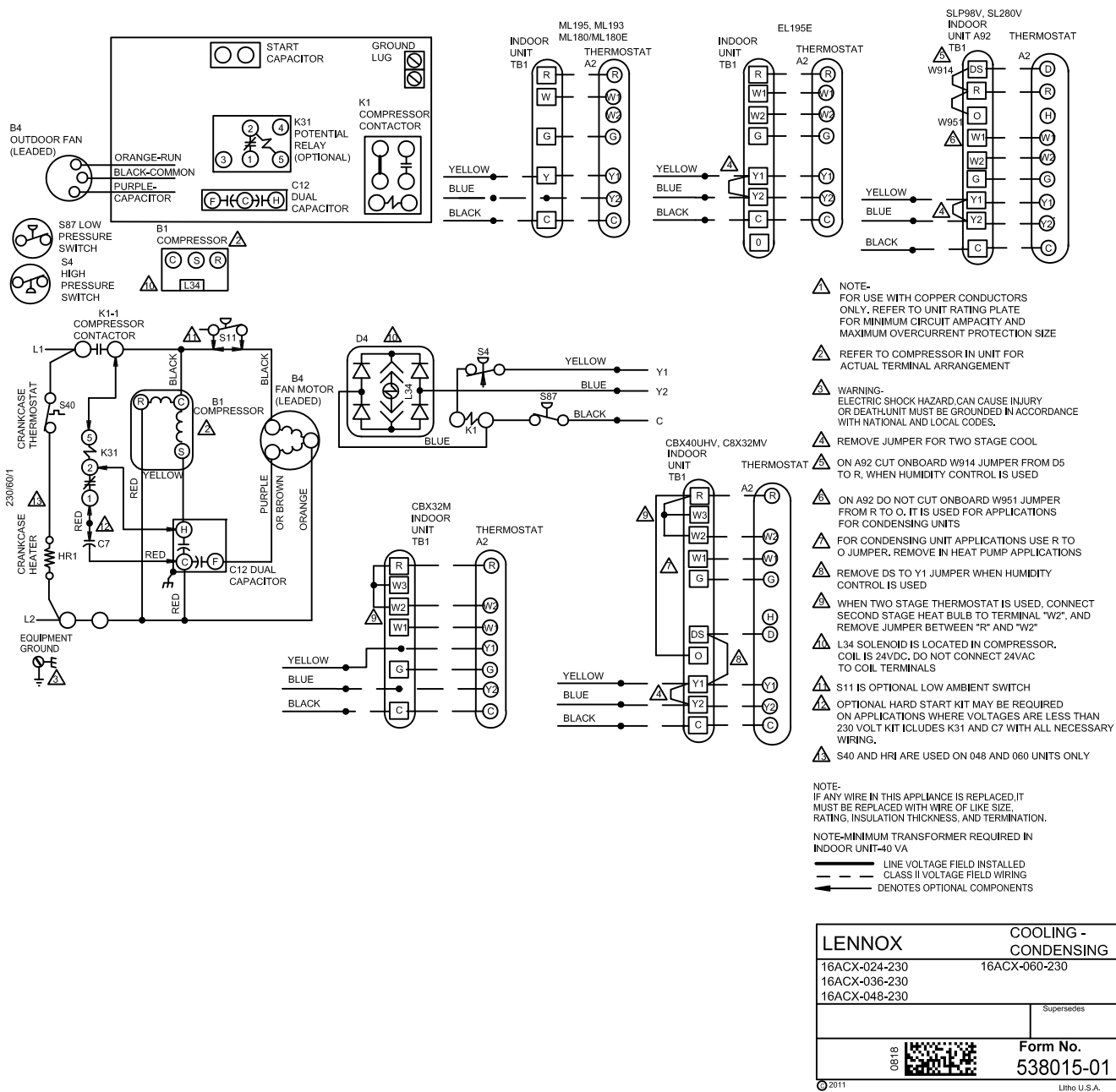
FIGURE 13. Typical Field Wiring
