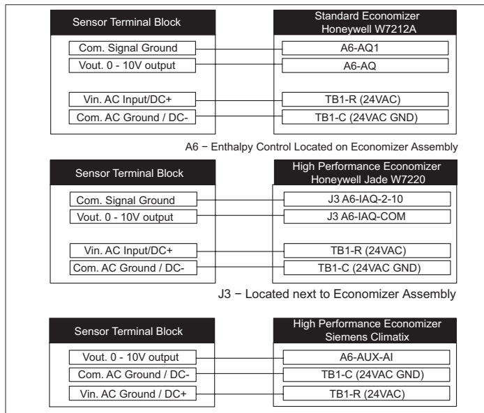
Figure 3. Field Wiring for KC/KG/KH, ZC/ZG/ZH and ELA units without Unit Controller
