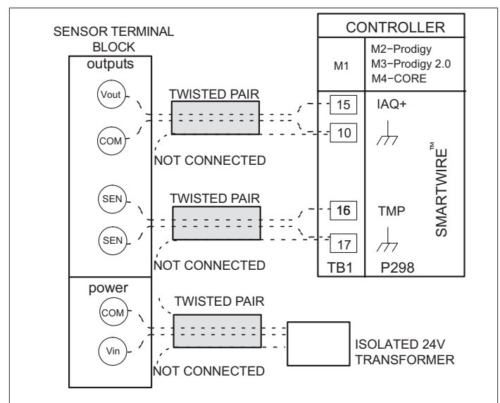
Figure 2. Field Wiring - 150' (46m) or Longer Runs
