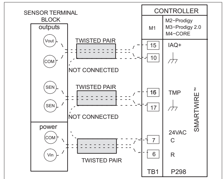
Figure 1. Field Wiring - 150' (46m) or Shorter Runs
