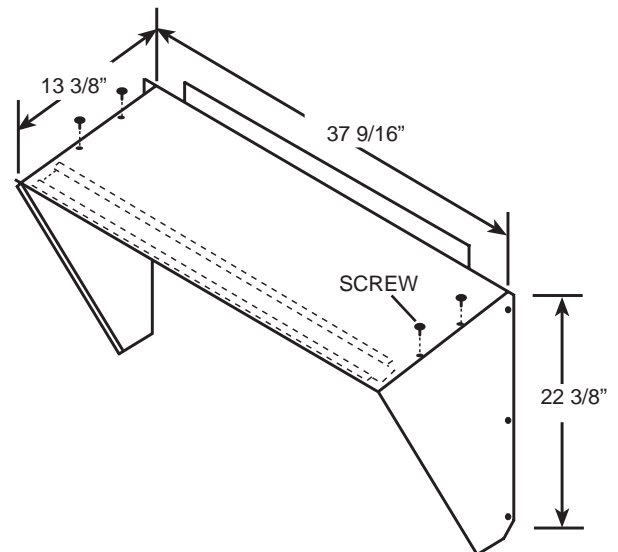
GRAVITY EXHAUST HOOD ASSEMBLED
