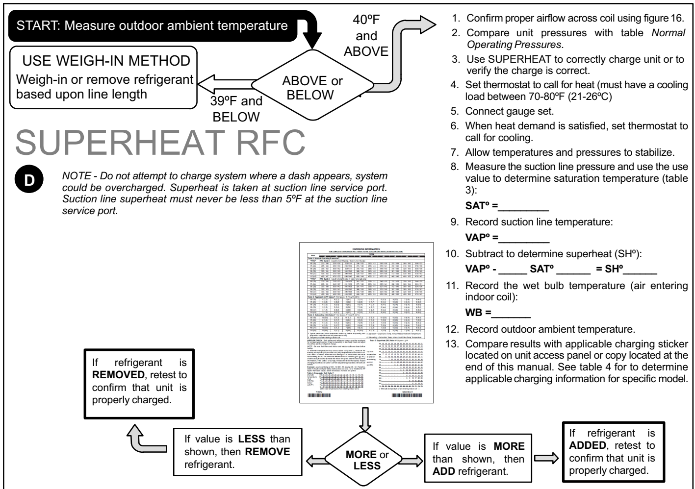
Figure 21. Using HFC-410A Superheat (Fixed Orifice) Charge Method
