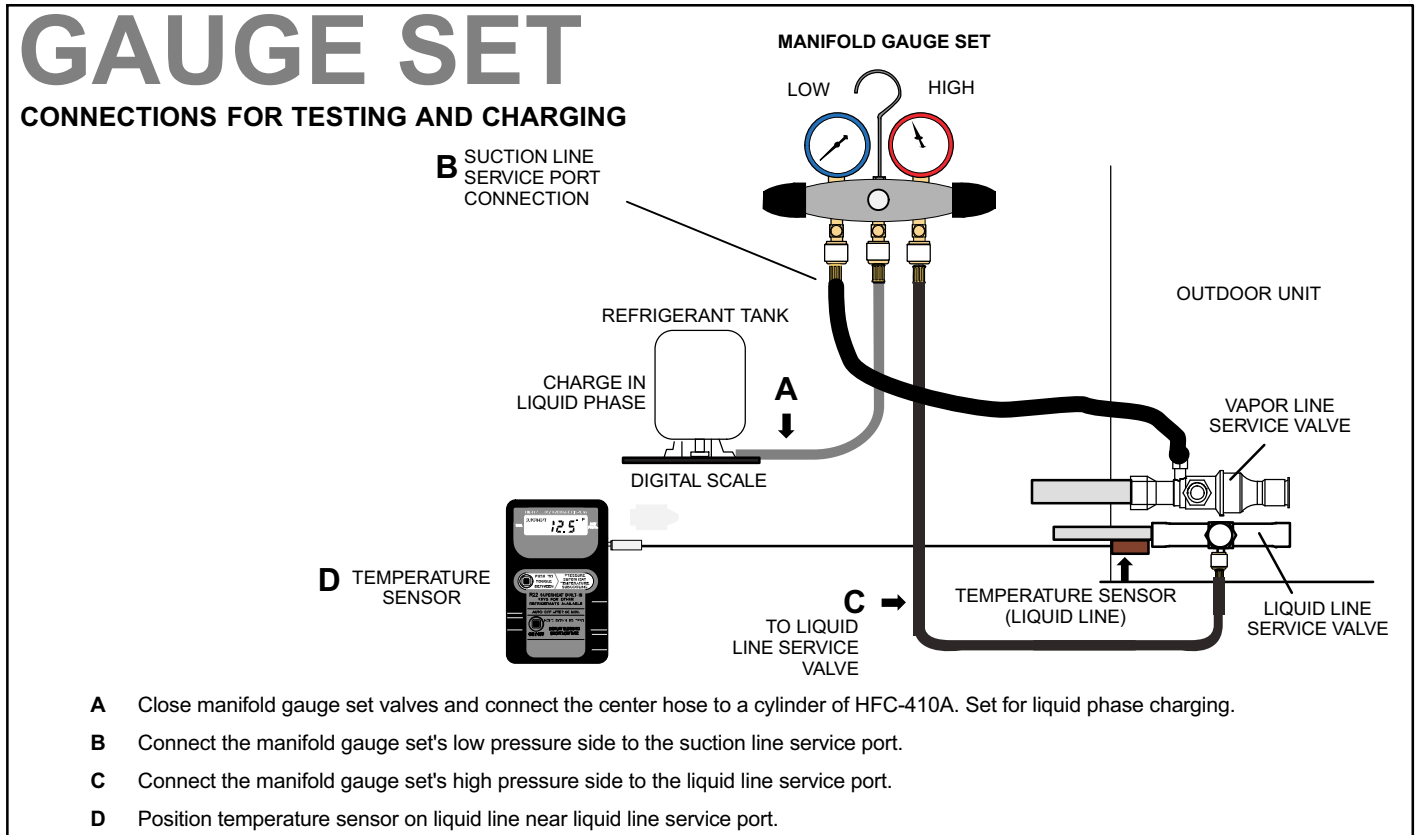
Figure 15. Gauge Set Setup and Connections
