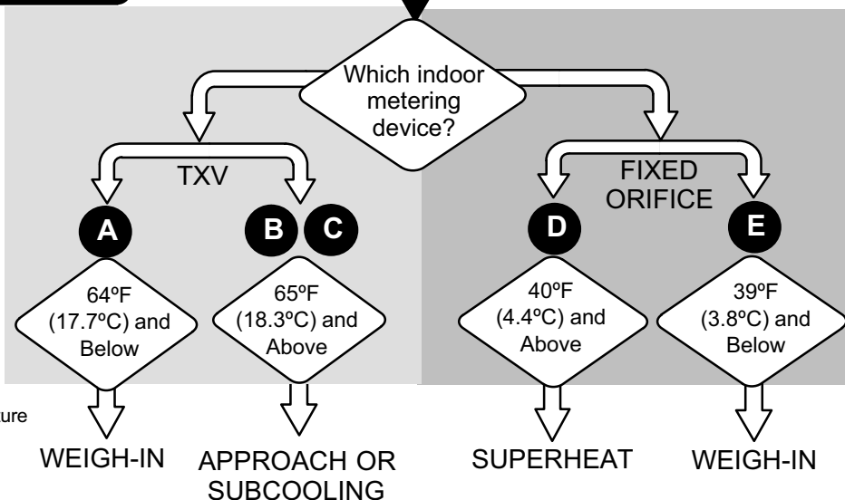
Figure 17. Determining Charge Method
