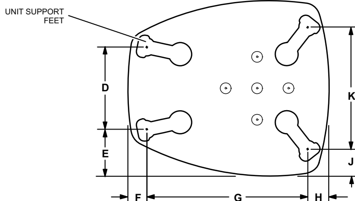
XC14-024-230-02 TO -060 BASE WITH ELONGATED LEGS
