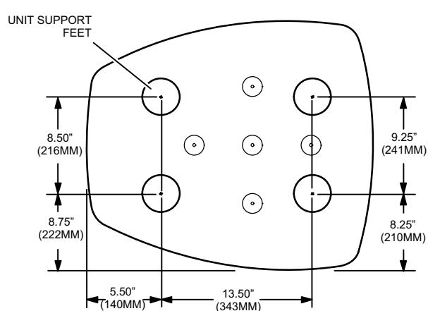
XC14-018-230-XX (All) and -024-01 BASE SECTION
