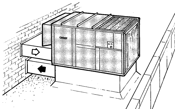
Rooftop Installation with Horizontal (End) Supply and Return Air System
