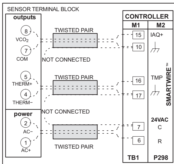
AC Power 3-Wire System
