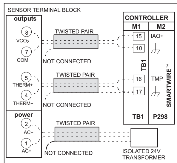
Isolated AC Power 4-Wire System
