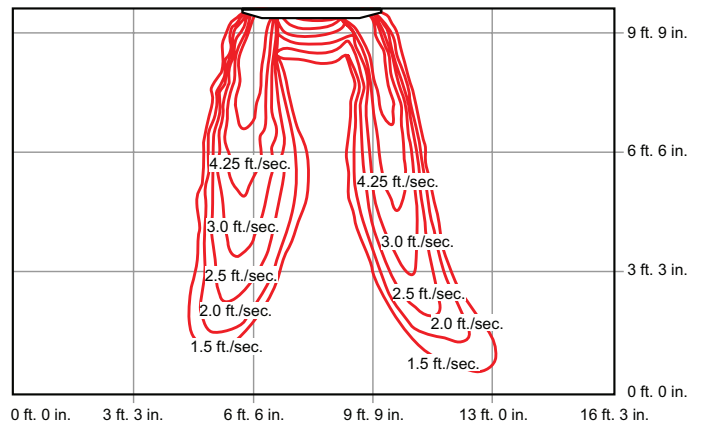
V22B012S4 - HEATING
