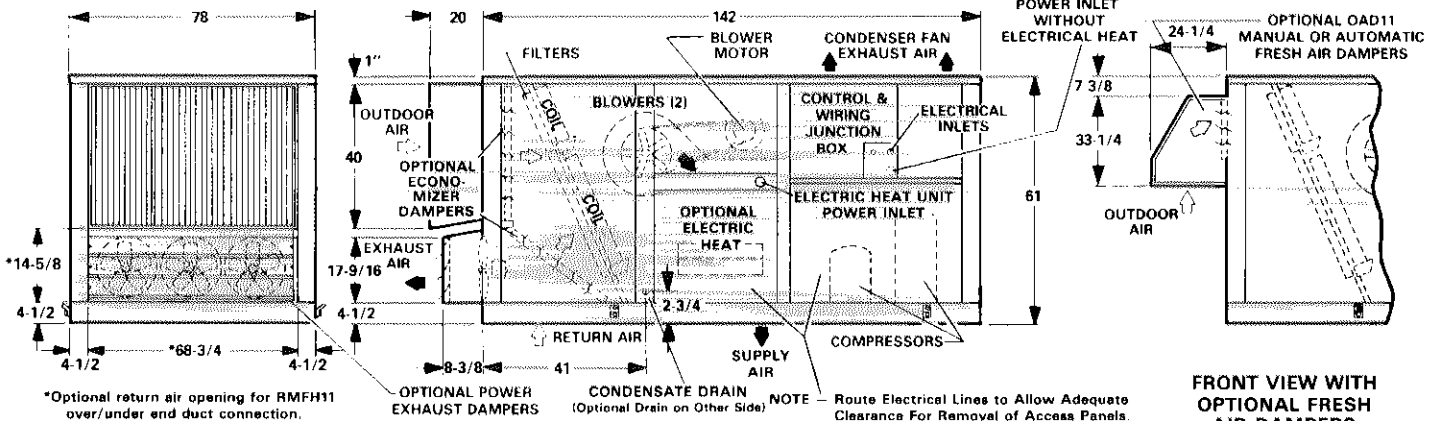
EXHAUST & OUTDOOR AIR INTAKE VIEW
