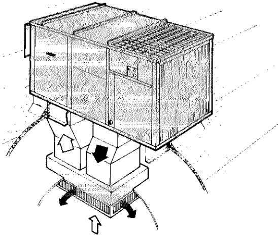
Rooftop Installation with Combination Ceiling Supply and Return Air System
