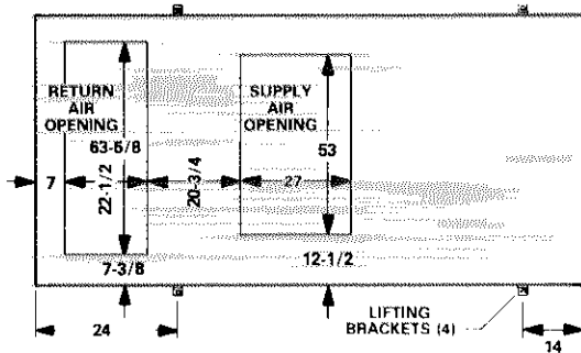
TOP VIEW BASE SECTION
