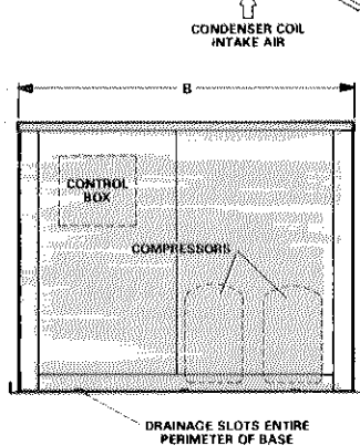
COMPRESSOR END VIEW
