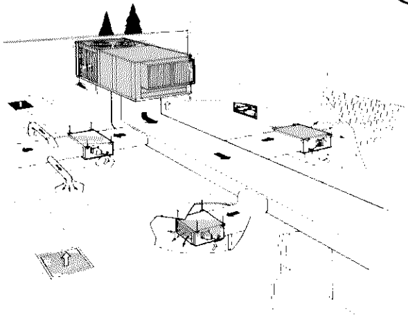
Rooftop Installation with Optional ZDB1 Blower Powered Mixing Damper Boxes.
