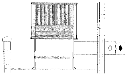
Horizontal Supply and Return Air (Side by Side) Duct Application
