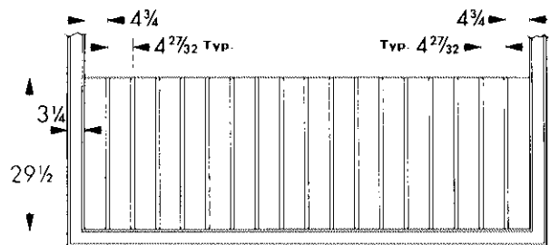
SUPPLY AIR CONNECTIONS FOR 18 OR LESS ZONES
