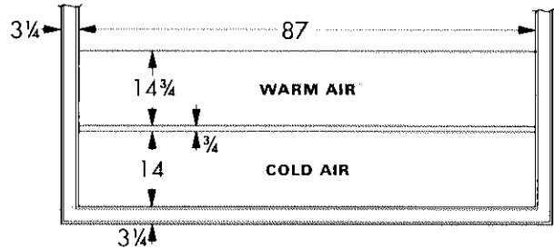
SUPPLY AIR CONNECTIONS FOR DOUBLE DUCT APPLICATIONS
