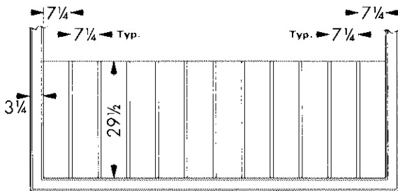
SUPPLY AIR CONNECTIONS FOR 12 OR LESS ZONES
